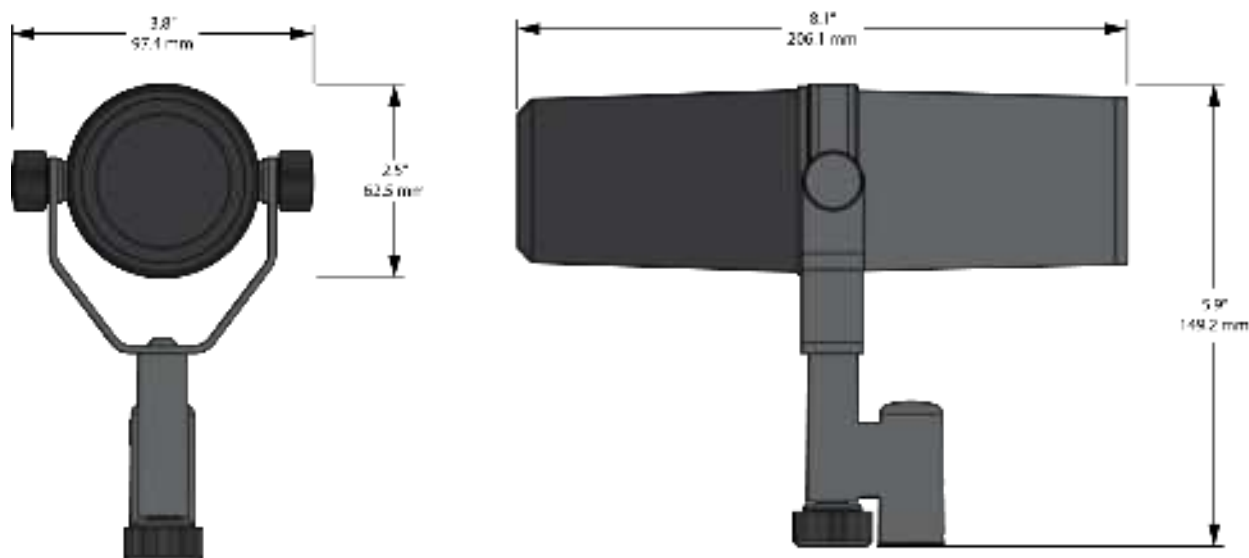
Overall Dimensions
