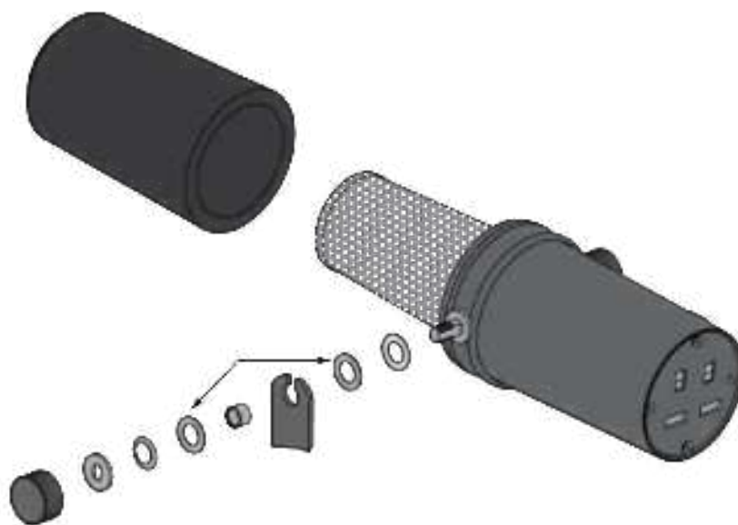
Mounting Assembly - Exploded View
