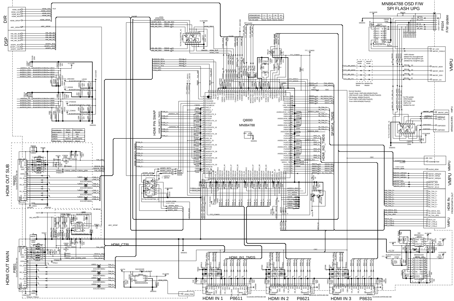
SCHEMATIC DIAGRAM (PART-10) VIDEO PROCESSOR SECTION
