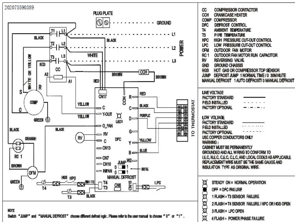
Outdoor Unit Wiring Diagram for H/P Systems(208/230V 3P 60Hz).
