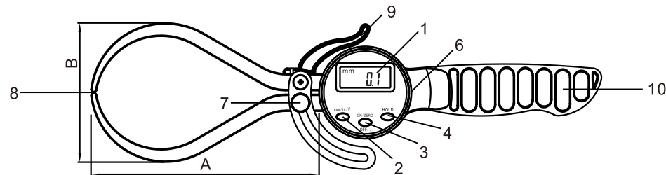
Type:B with Handle
