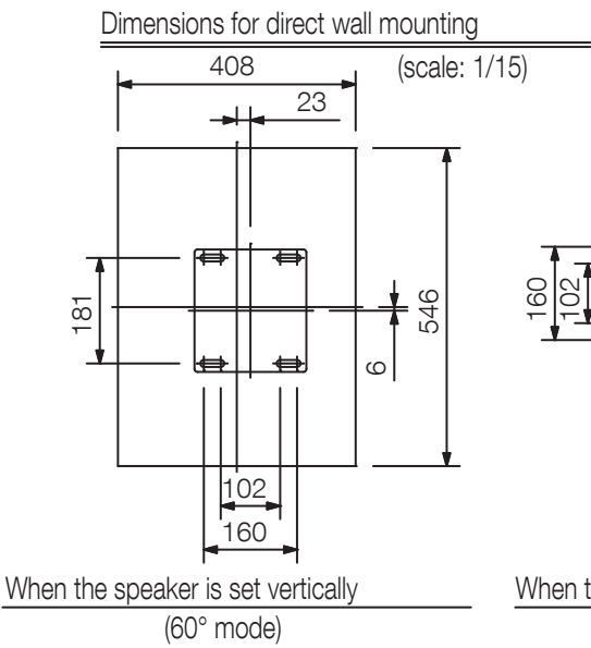
Example for direct wall mounting (scale: 1/15)
