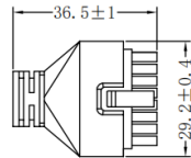
Small 5557-16P
