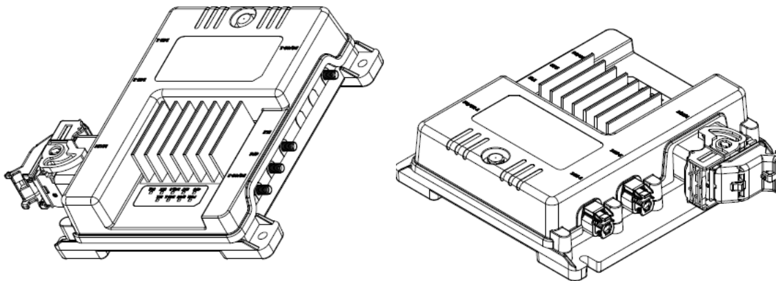
Fig. 2.1 Front/Rear View
