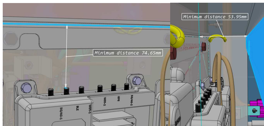
Fig. 4.2 Mounting Example of TGU
