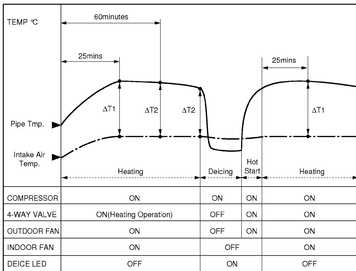
(DEICING DIAGRAM)
