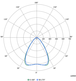
Polar Normal (separate) - SM350CI - 910925868353
