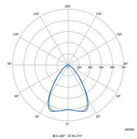
Polar Normal (separate) - SM350CI - 910925868390
