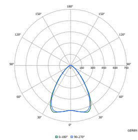
Polar Normal (separate) - SM350CI - 910925868377
