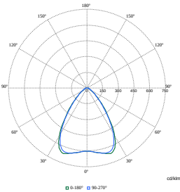
Polar Normal (separate) - SM350CI - 910925868355
