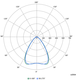
Polar Normal (separate) - SM350CI - 910925868352
