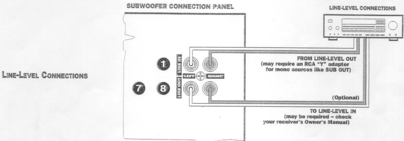
Figure 3. Connecting left and right line-level outputs of an A/V receiver to left and right line-level inputs of the Cerwin-Vega subwoofer. Remember to maintain left to left, right to right, (+) to (+) and (-) to (-) connections!
