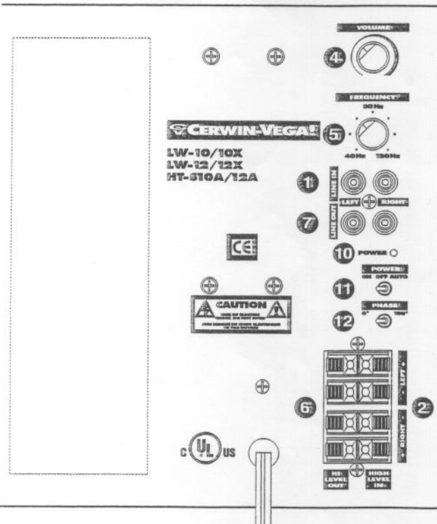
Figure 2. Connection panel for the HT-S10A, HT-S12A, LW-10/10X, and LW-12/12X.
