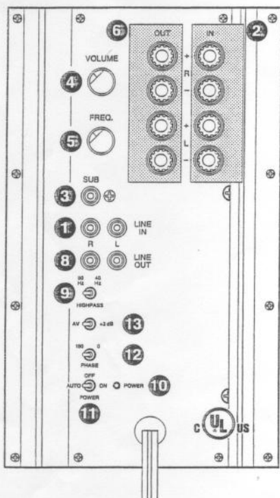
Figure 1. Connection panel for the HT-S15A and LW-15/15X.
