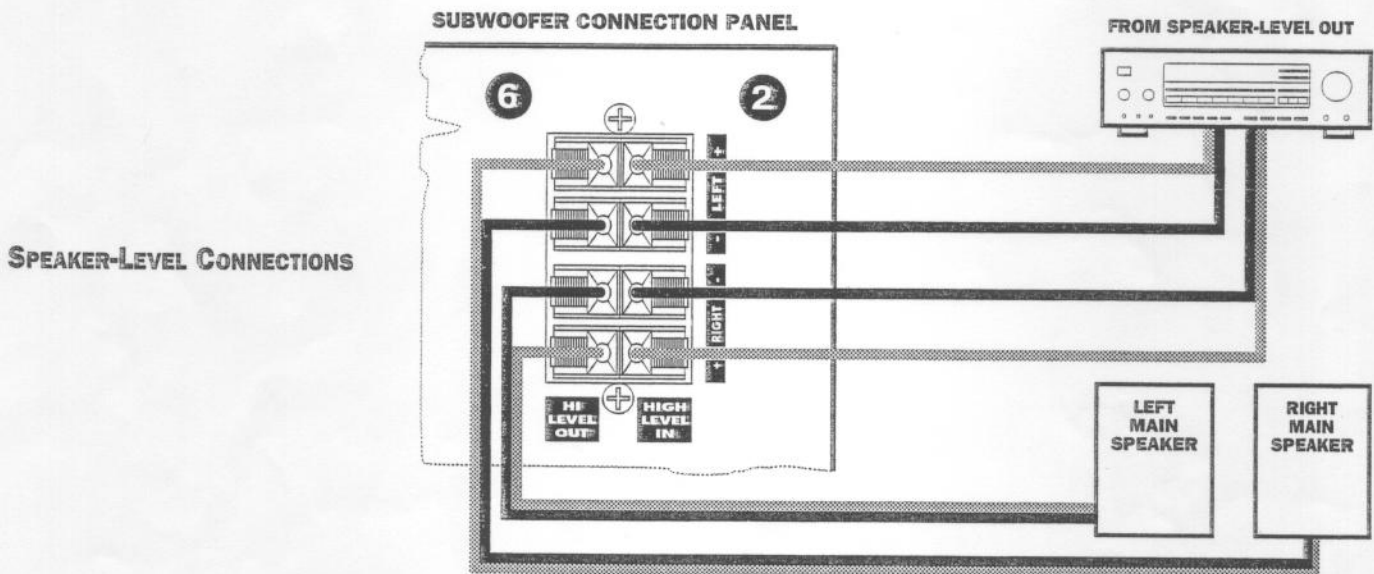
Figure 4. Connecting left and right speaker-level outputs of an A/V receiver to left and right speaker-level inputs of the subwoofer. Then connect left and right speaker-level outputs of the subwoofer, with the main left and right speakers of your system. Remember to maintain left to left, right to right, (+) to (+) and (-) to (-) connections.
