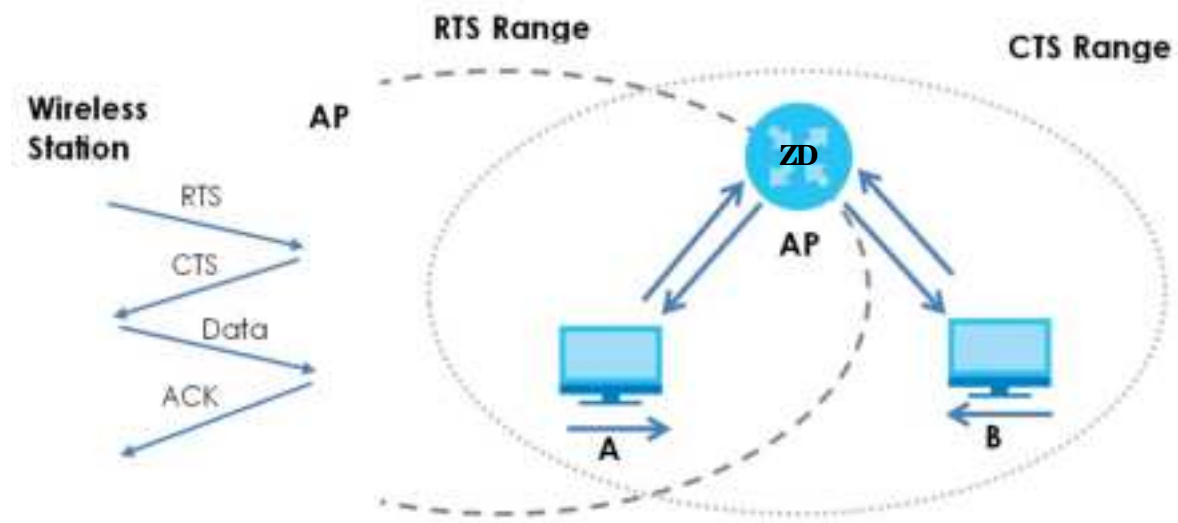
Figure 210 RTS/CTS
