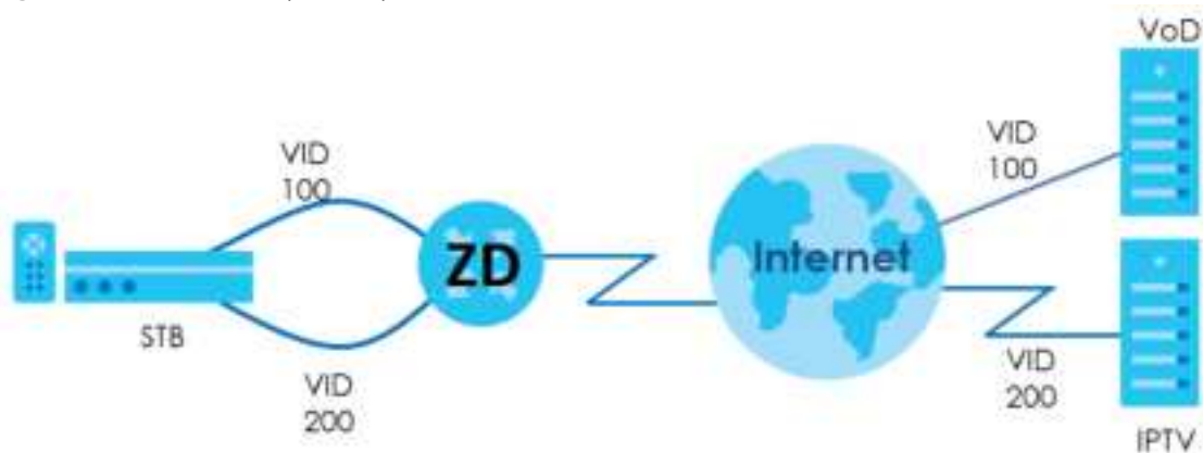
Figure 141 VLAN Group Example
