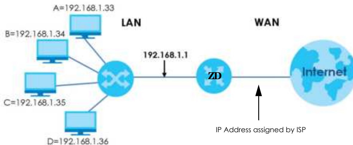
Figure 137 Multiple Servers Behind NAT Example
