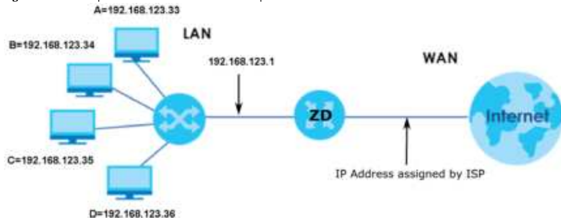
Figure 127 Multiple Servers Behind NAT Example
