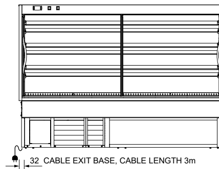
REAR ELEVATION
