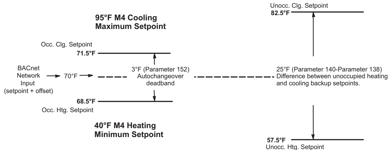
Figure 1. CORE Unit Controller Default Setpoint Example (Room Sensor Installed)
