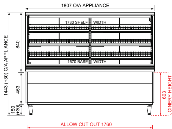
FRONT ELEVATION
