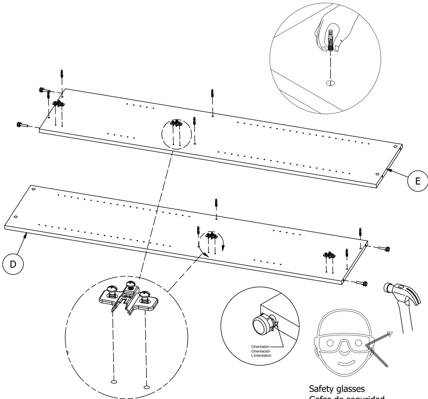
Mounting Plate
