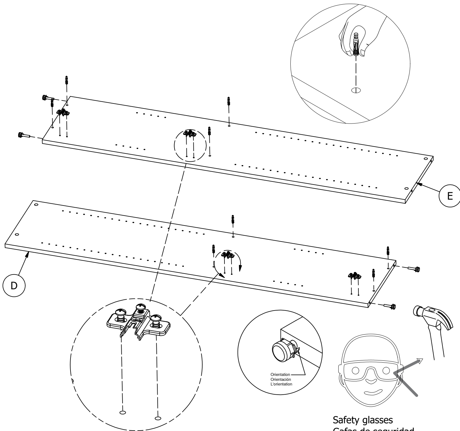
Mounting Plate
