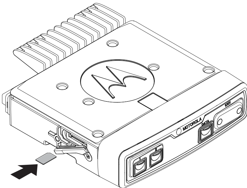
Figure 14: Inserting the TETRA SIM (mini-SIM) Card (MXM7000 with 2-DIN Configuration)
