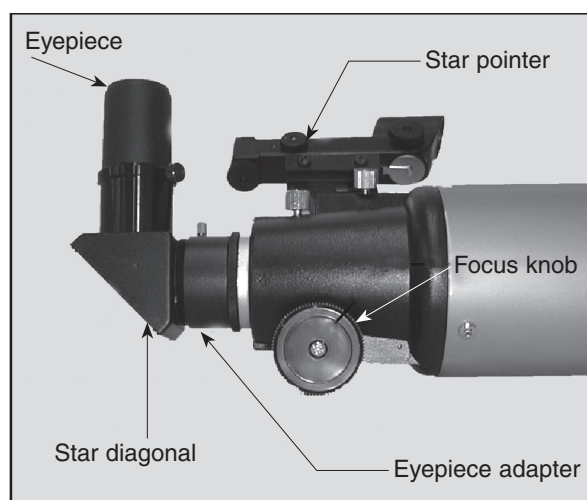
Figure 2-3. Visual accessories for the StarSeeker 100mm
