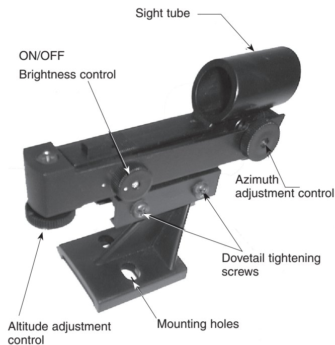
Figure 2-4. The Star Pointer finderscope with bracket
