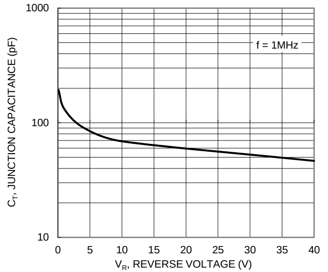
Figure 2. Typical Junction Capacitance
