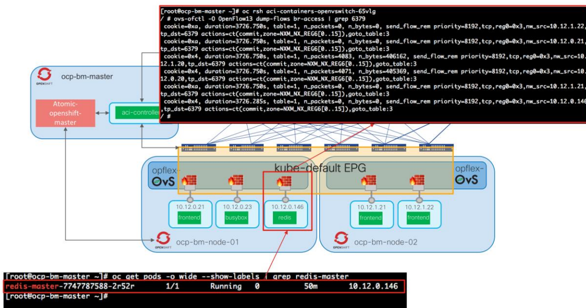
Figure 60: Host Protection Policy implemented as OVS OpenFlow rules
