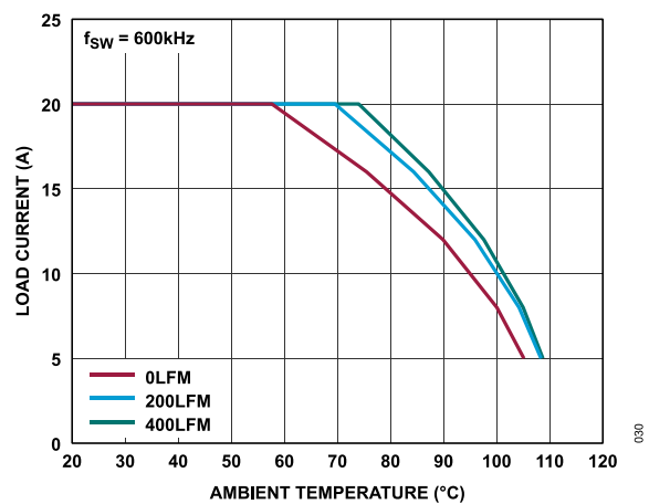
Figure 30. 12V to 1V Derating Curve, No Heat Sink
