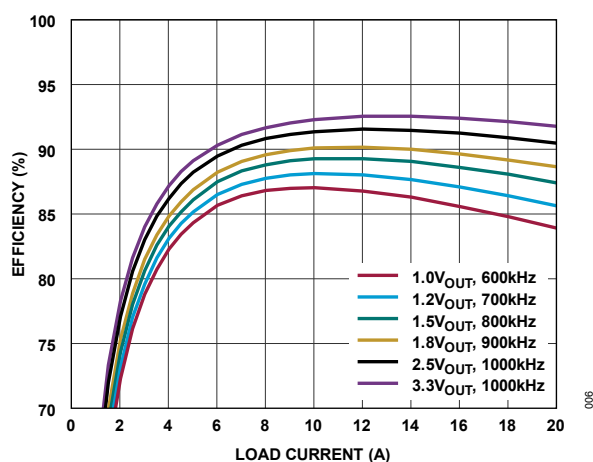
Figure 6. Efficiency vs. Load Current from 12V IN
