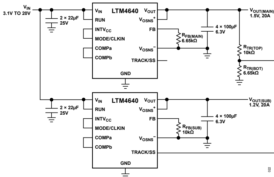
Figure 22. Example Schematic of Ratio Metric Output Voltage Tracking
