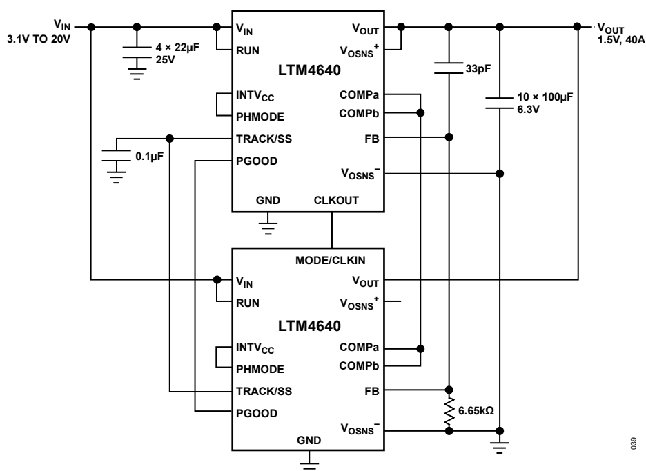
Figure 39. 3.1V IN to 20V IN , Two Phases, 1.5V at 40A Design
