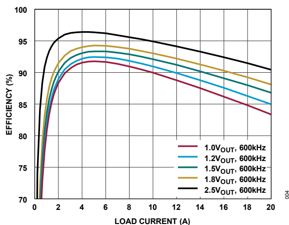
Figure 4. Efficiency vs. Load Current from 3.3V IN
