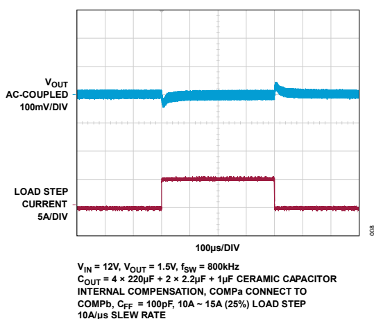
Figure 8. 1.5V OUT Transient Response
