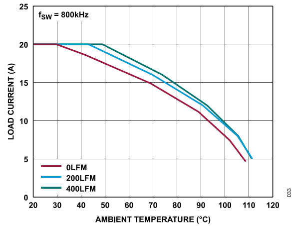
Figure 33. 5V to 3.3V Derating Curve, No Heat Sink
