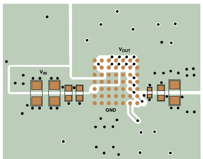
Figure 36. Recommended PCB Layout
