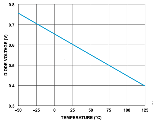
Figure 24. Diode Voltage V_D vs. Temperature T(^{\circ}\text{C})
