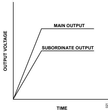
Figure 21. Output Ratio Metric Tracking Waveform
