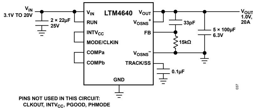
Figure 37. 3.1V IN to 20V IN , 1V Output at 20A Design
