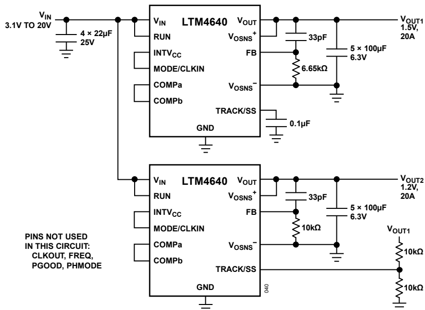
Figure 40. 3.1V IN to 20V IN , 1.2V and 1.5V with Coincident Tracking
