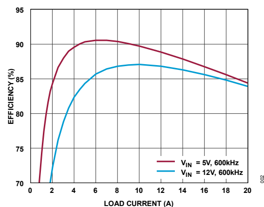
Figure 2. 1V OUT Efficiency vs. Load Current
