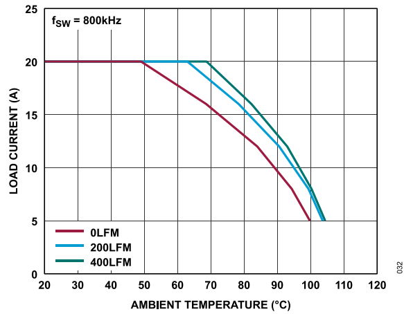
Figure 32. 12V to 1.5V Derating Curve, No Heat Sink
