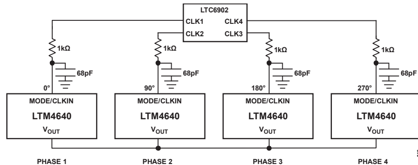
Figure 19. 4-Phase Operation with an External Clock IC and Low-Pass Filters
