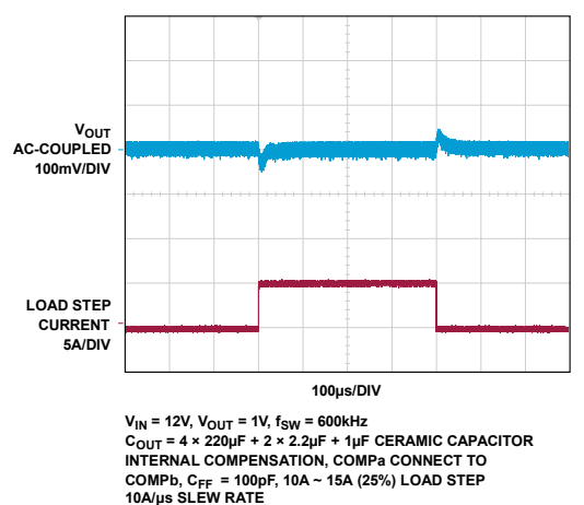
Figure 7. 1V OUT Transient Response
