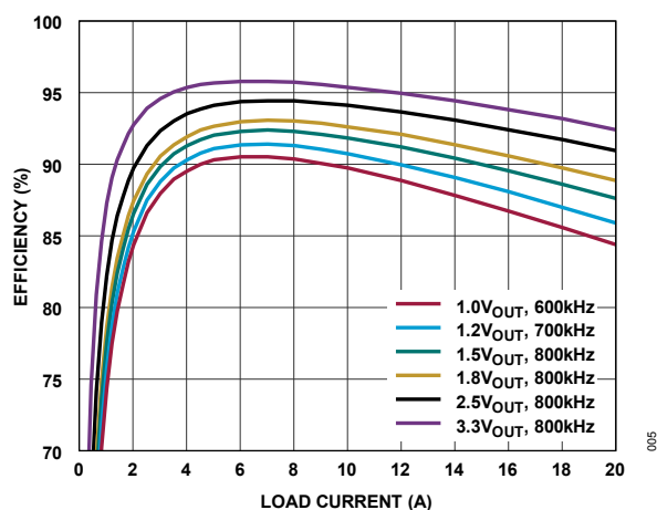
Figure 5. Efficiency vs. Load Current from 5V IN
