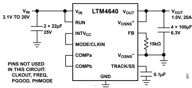
Figure 1. 20A, 1V OUT DC-to-DC Step-Down \mu Module Regulator
