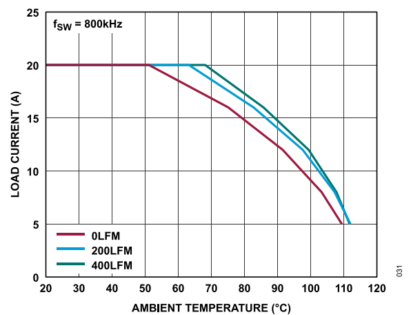
Figure 31. 5V to 1.5V Derating Curve, No Heat Sink
