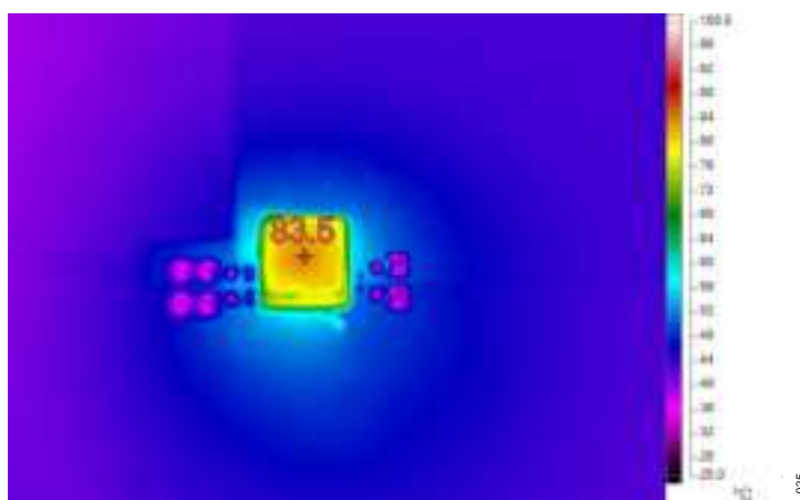
Figure 35. Thermal Image at 12V IN , 1V OUT at 20A, 600kHz, 21°C Ambient Temperature, without Airflow and Heat Sinking
