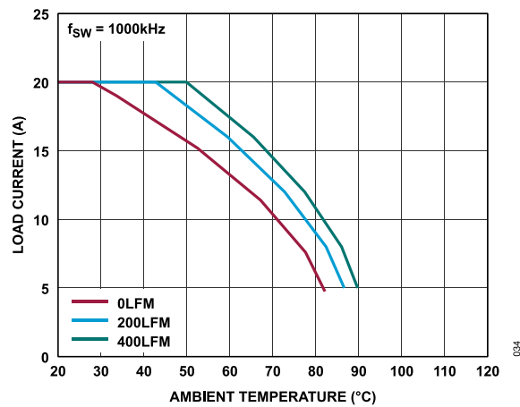
Figure 34. 12V to 3.3V Derating Curve, No Heat Sink
