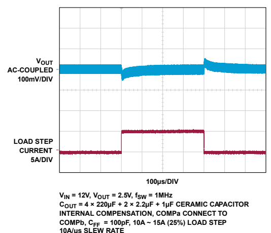
Figure 9. 2.5V OUT Transient Response
