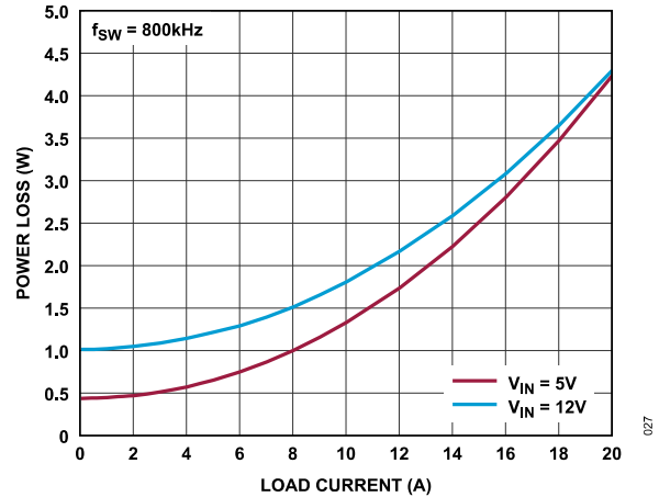
Figure 27. Power Loss at 1.5V Output
