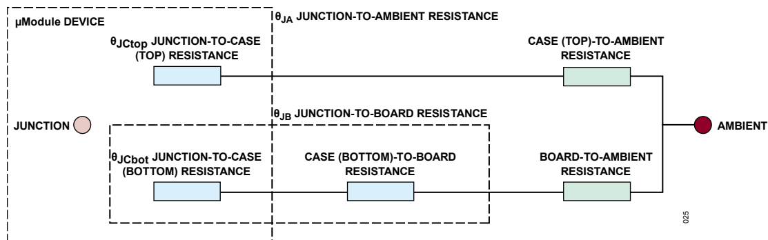
Figure 25. Graphical Representation of JESD51-12 Thermal Coefficients
