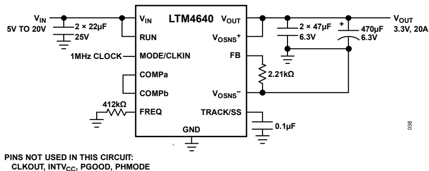
Figure 38. 5V IN to 20V IN , 3.3V Output with 1MHz External Clock
