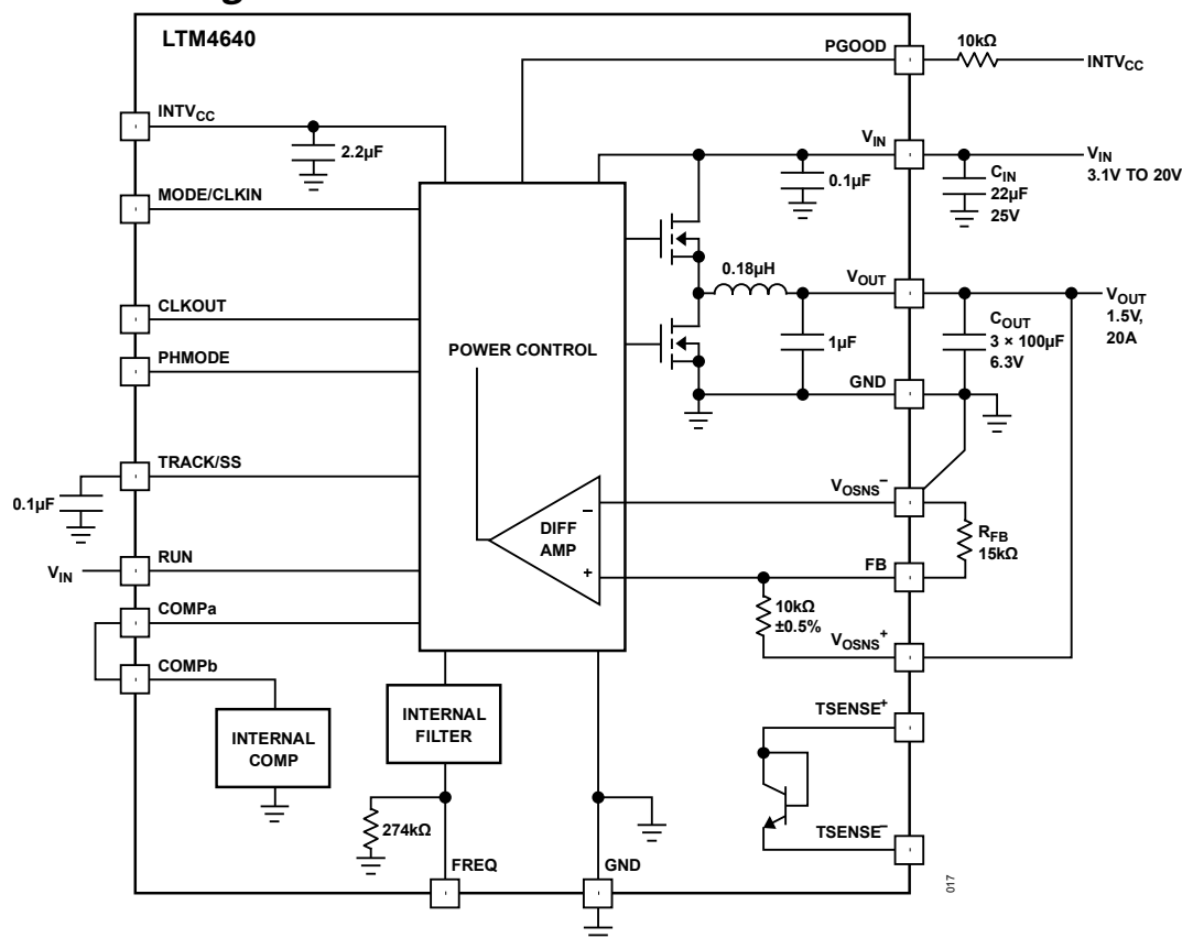
Figure 17. LTM4640 Simplified Block Diagram
