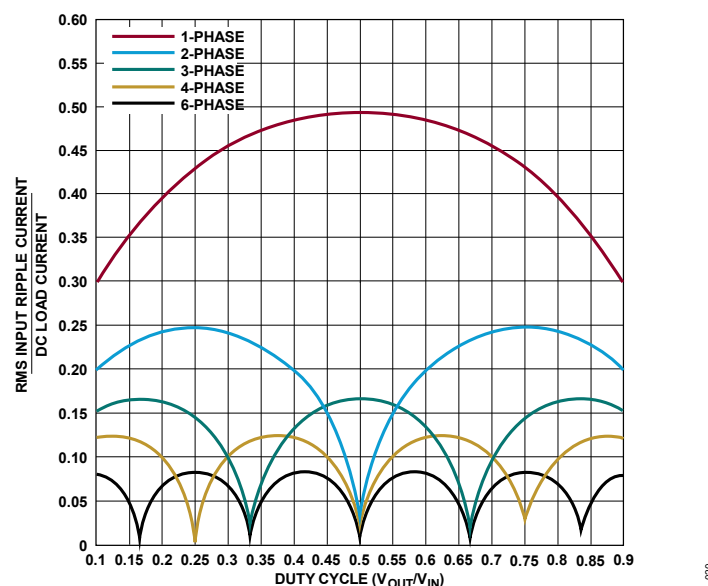
Figure 20. The RMS Input Ripple Current to DC Load Current Ratio as a Function of the Duty Cycle
