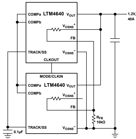
Figure 18. 2-Phase Parallel Configurations
