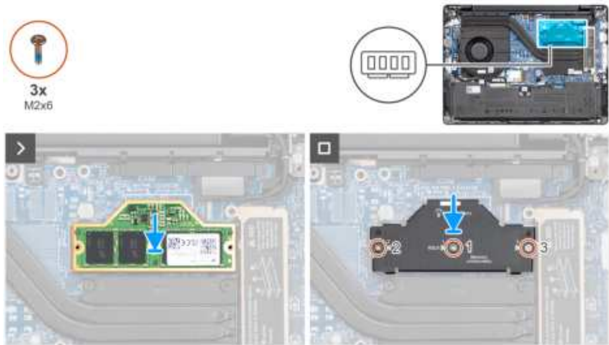
Figure 19. Installing the memory module
