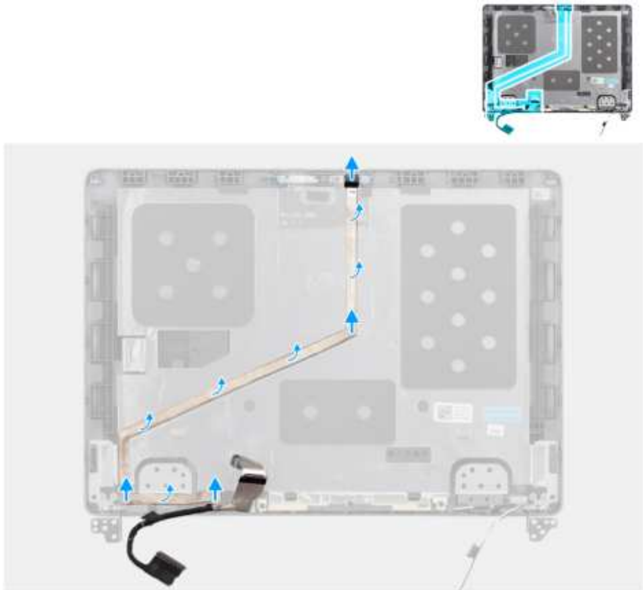
Figure 65. Removing the display cable
