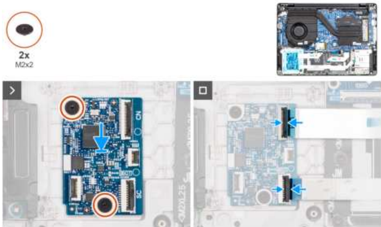
Figure 35. Installing the USH board
