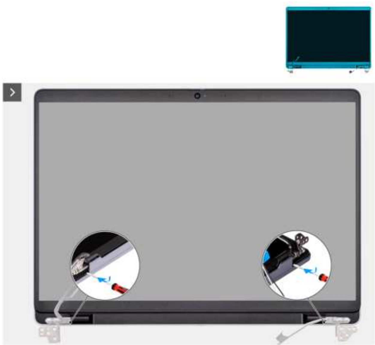
Figure 49. Removing the display bezel
