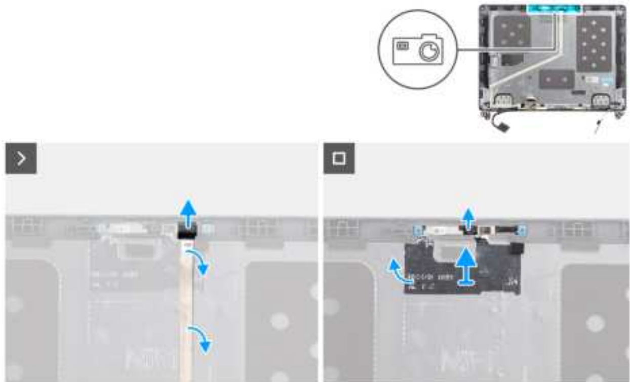
Figure 67. Removing the camera
