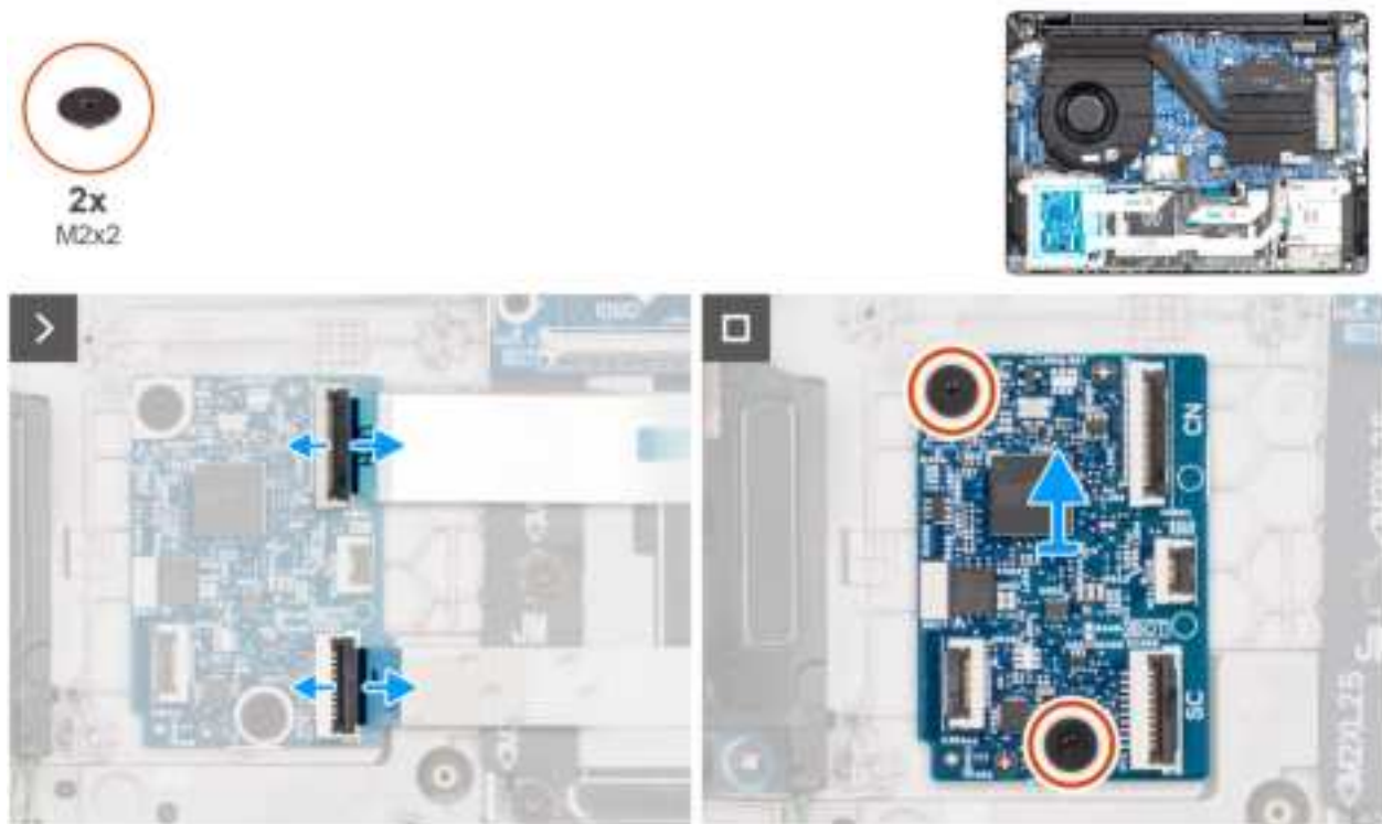
Figure 34. Removing the USH board
