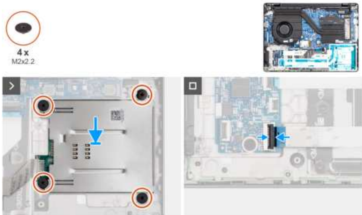
Figure 37. Installing the smart-card reader
