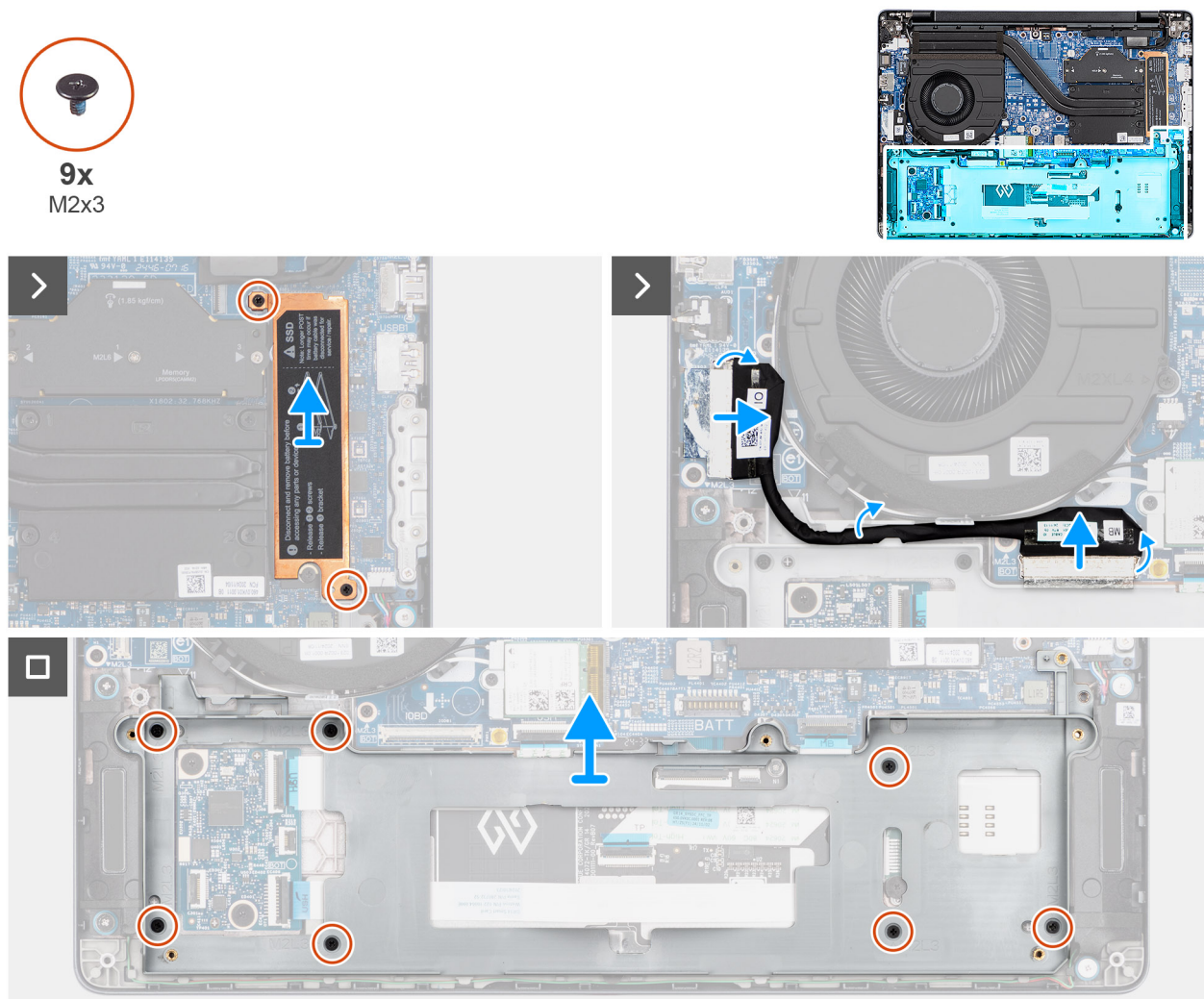
Figure 32. Removing the battery frame
