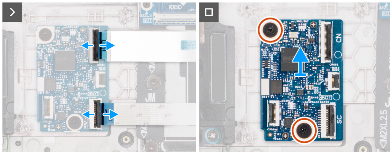
Figure 34. Removing the USH board
