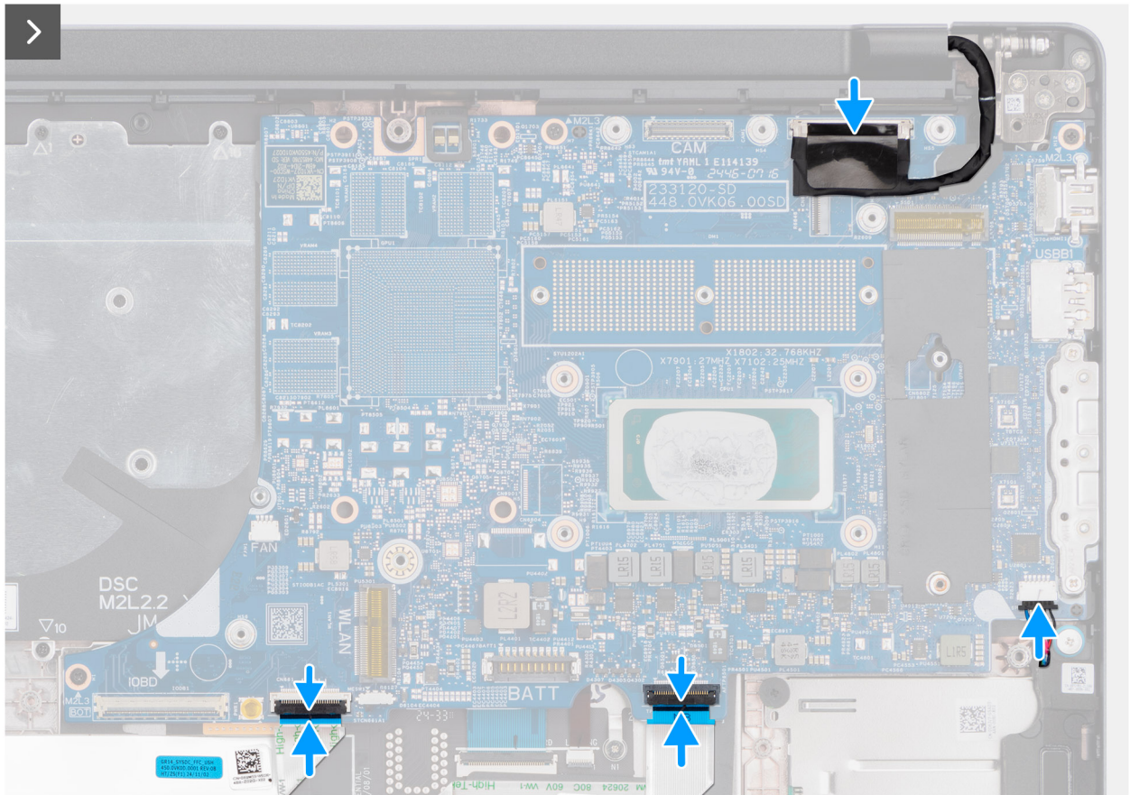
Figure 79. Installing the system board
