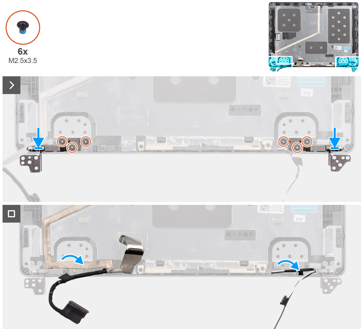
Figure 64. Installing the display hinges
