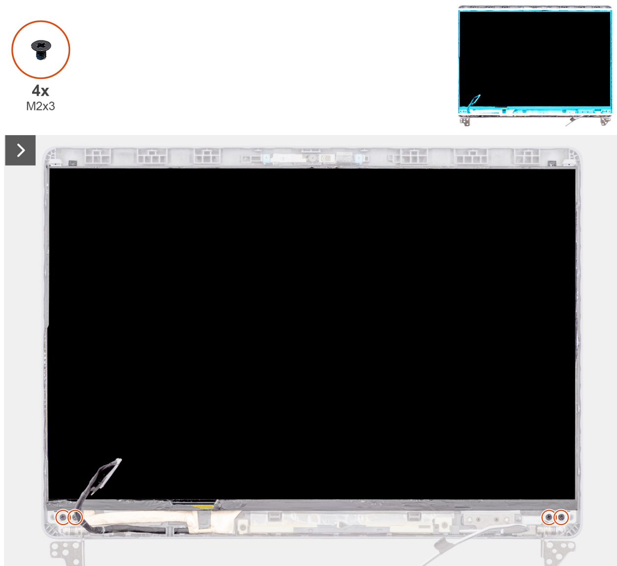
Figure 57. Removing the display panel
