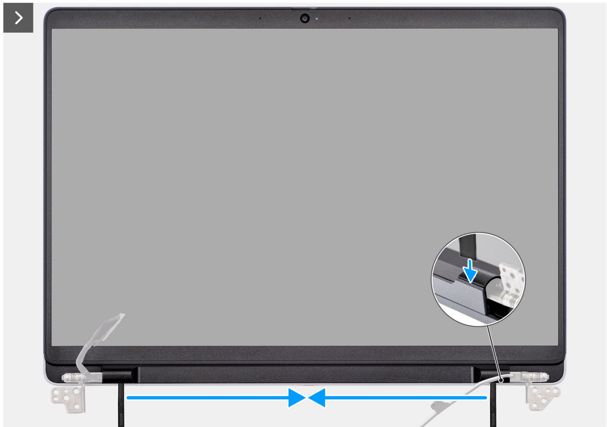
Figure 52. Removing the display bezel
