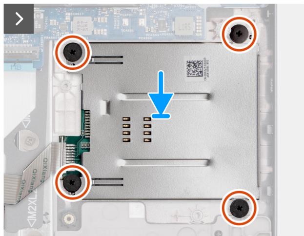
Figure 37. Installing the smart-card reader
