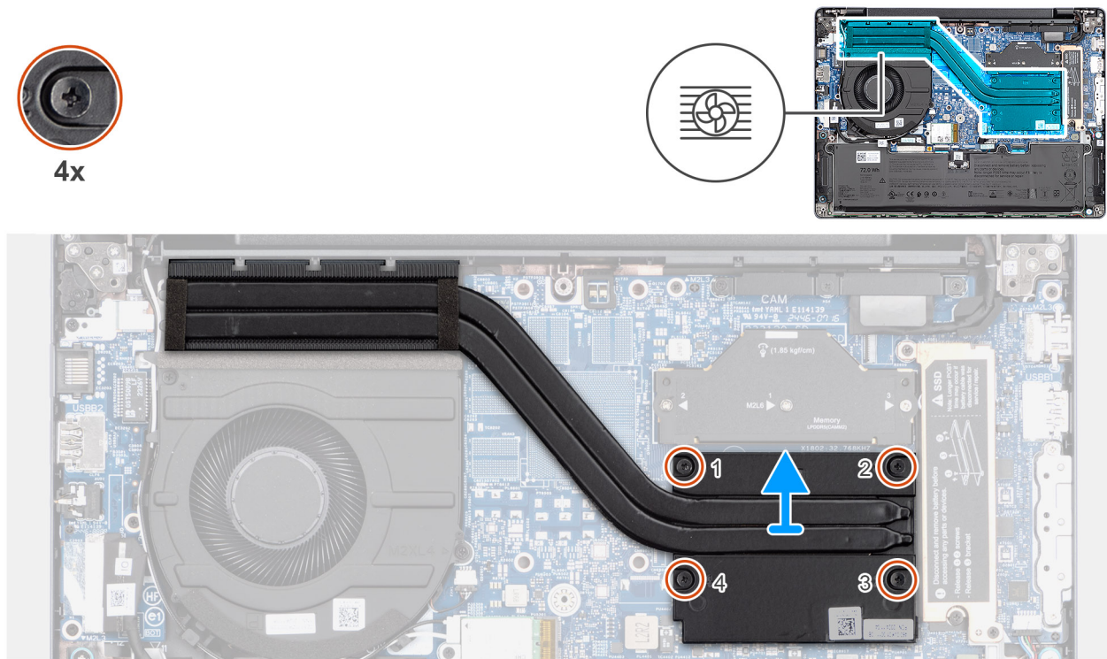
Figure 38. Removing the heat sink
