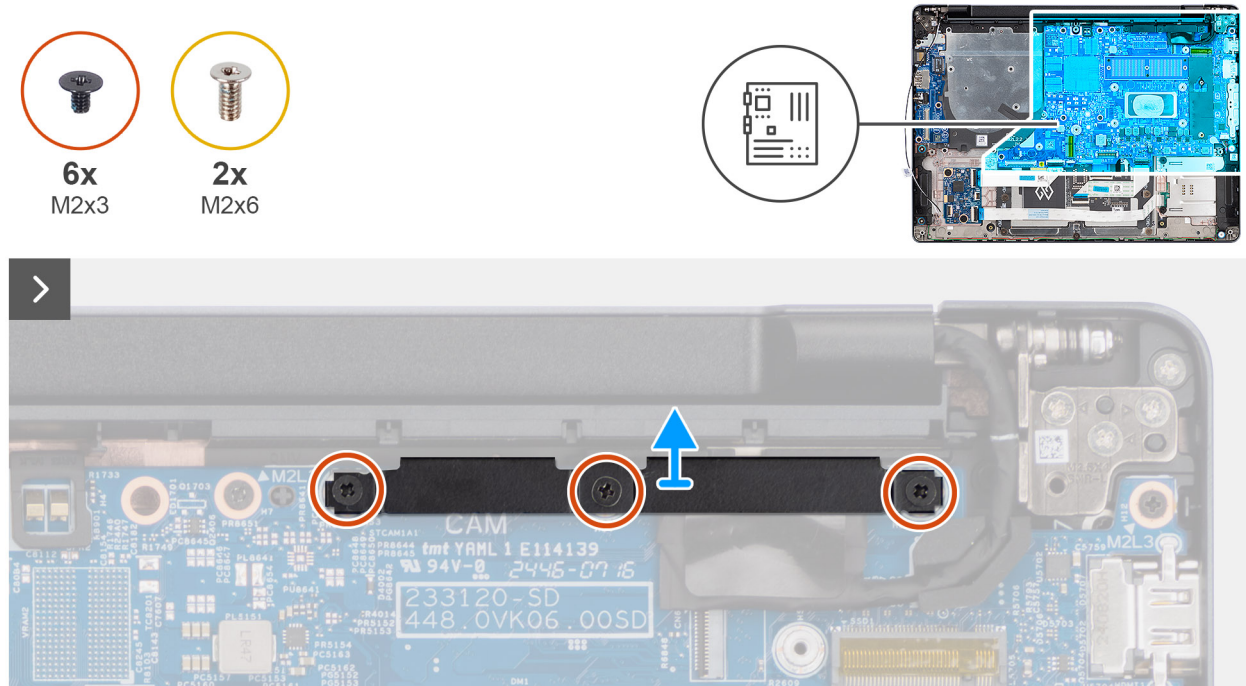
Figure 72. Removing the system board
