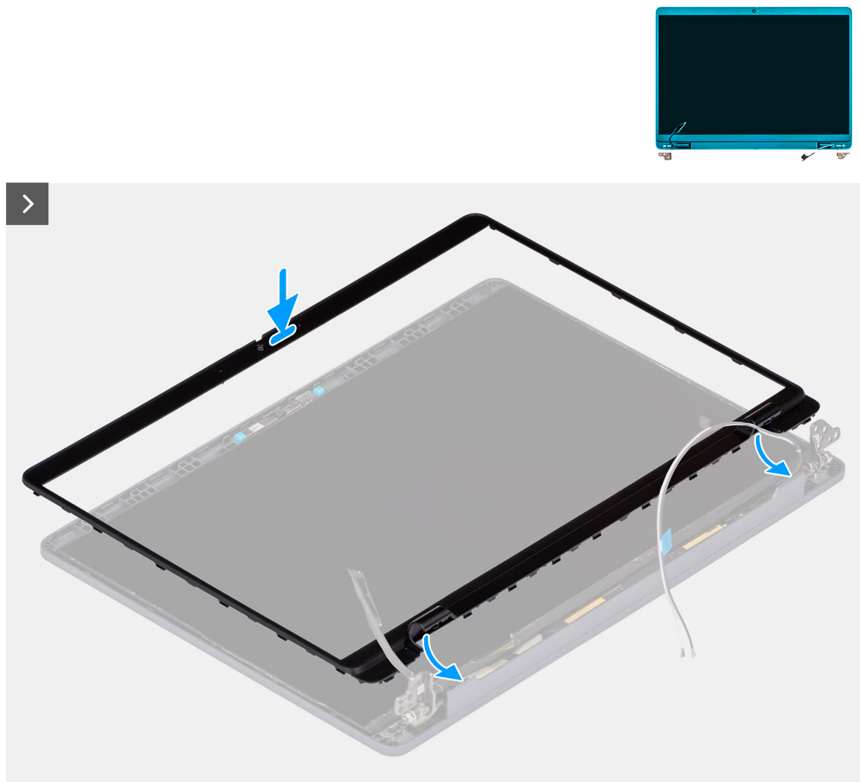
Figure 55. Installing the display bezel
