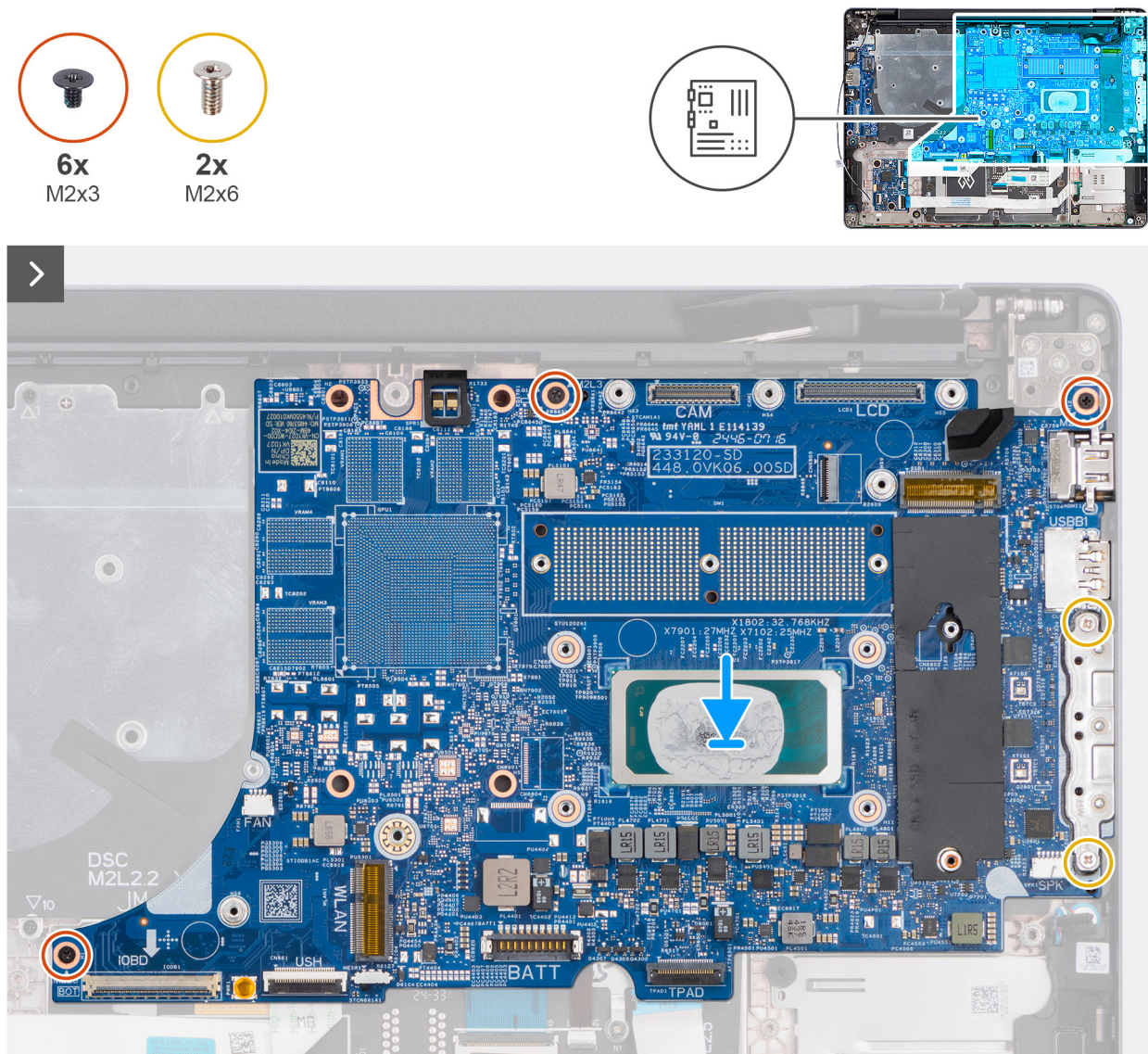
Figure 78. Installing the system board
