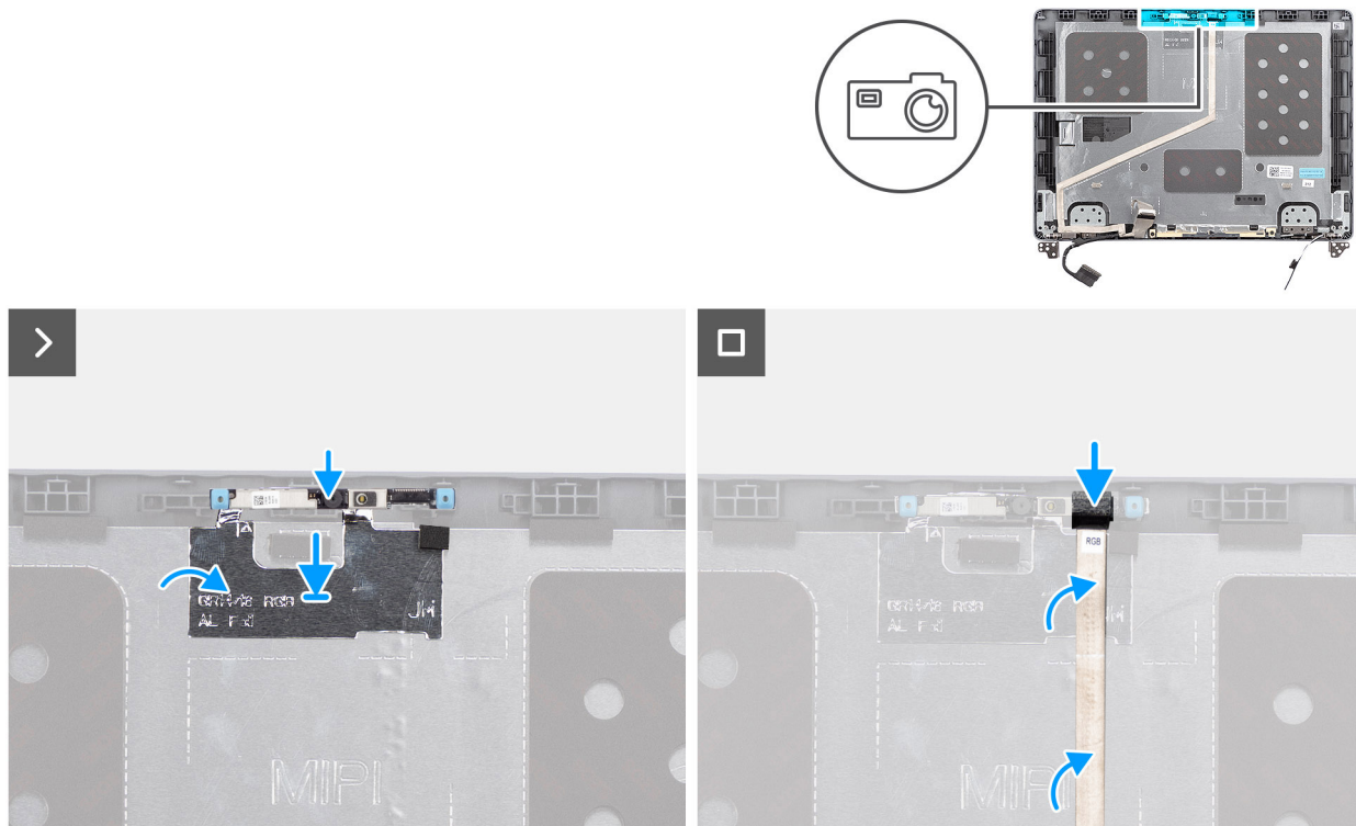
Figure 68. Installing the camera
