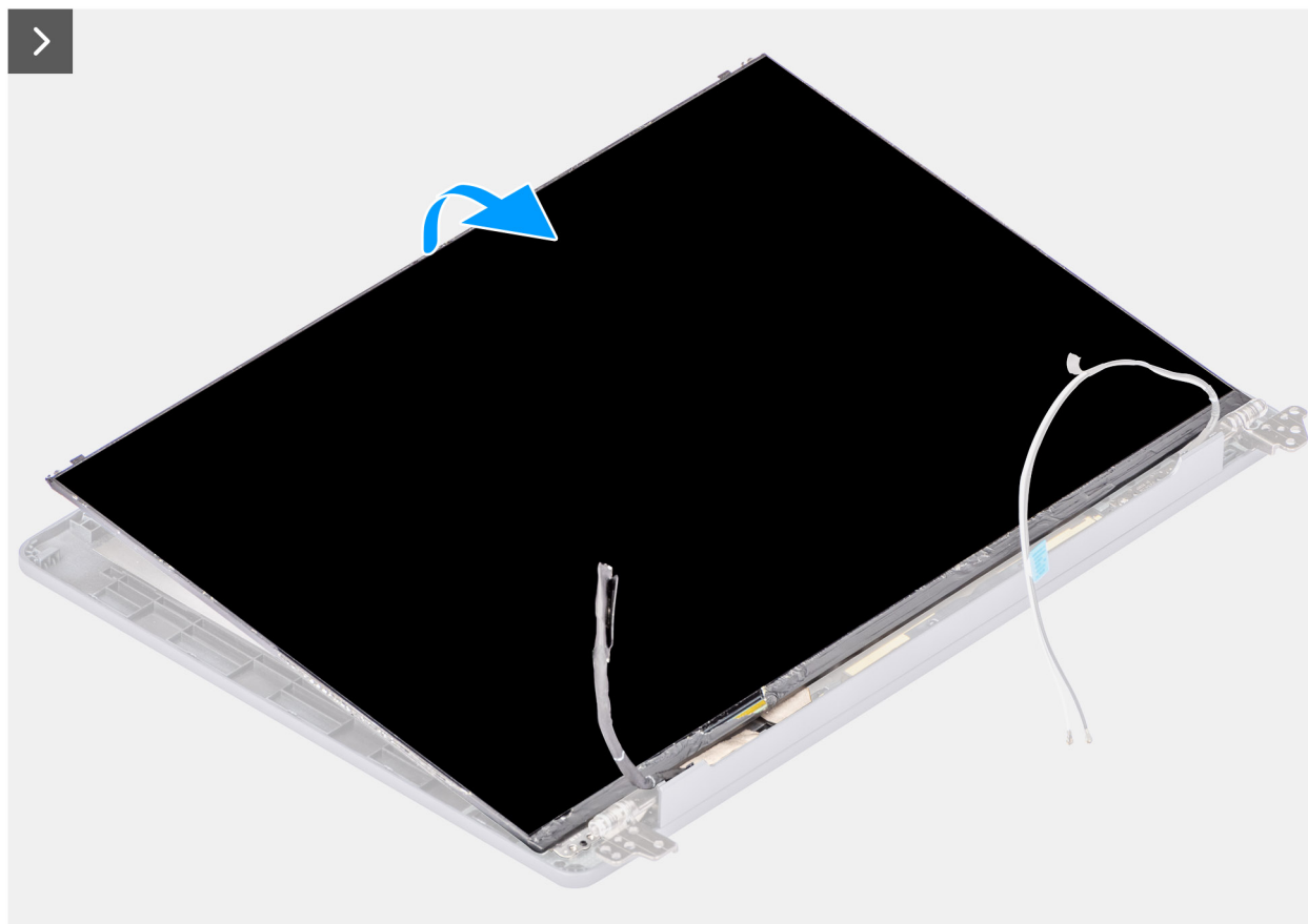
Figure 58. Removing the display panel
