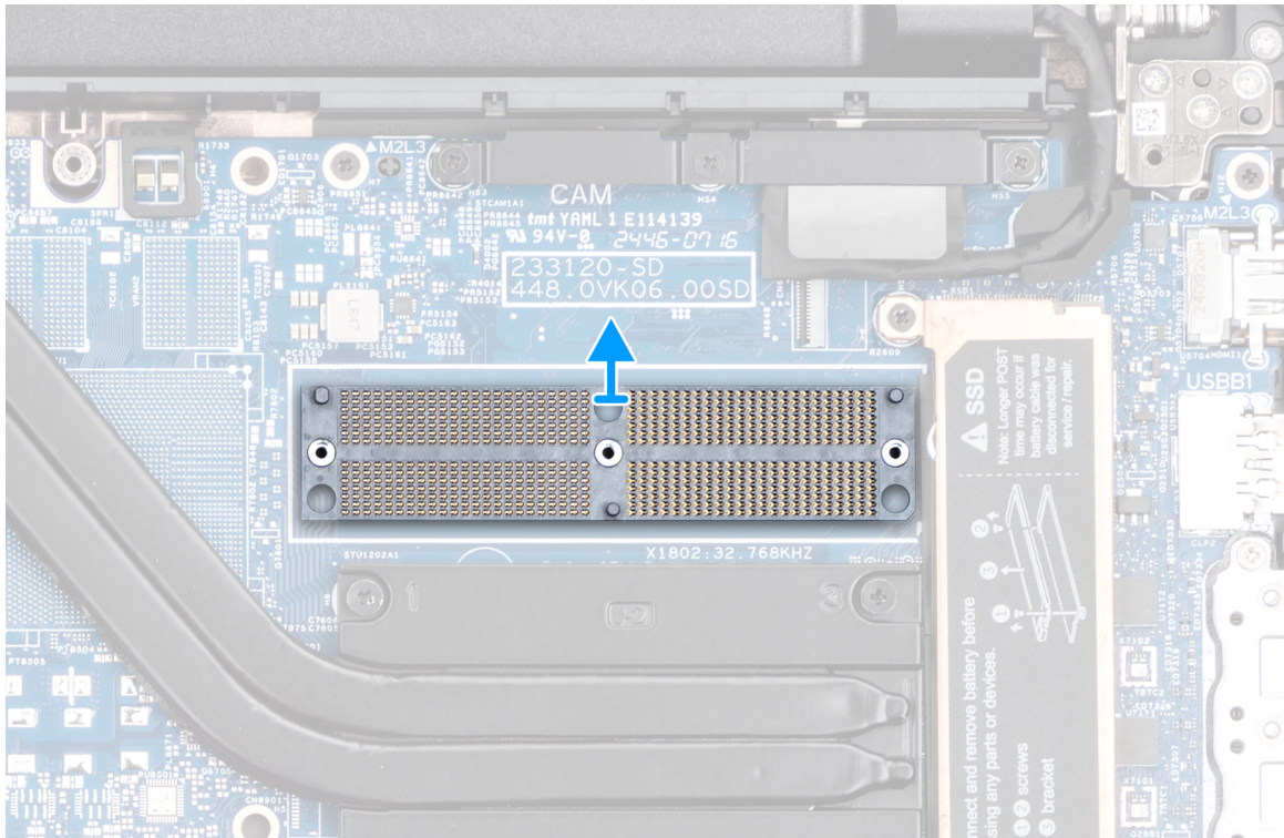
Figure 73. Removing the memory-module connector
