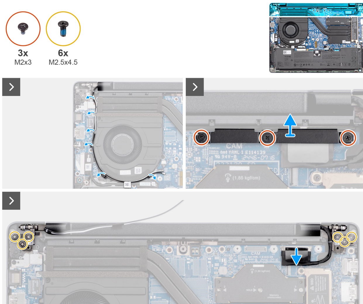
Figure 44. Removing the display assembly
