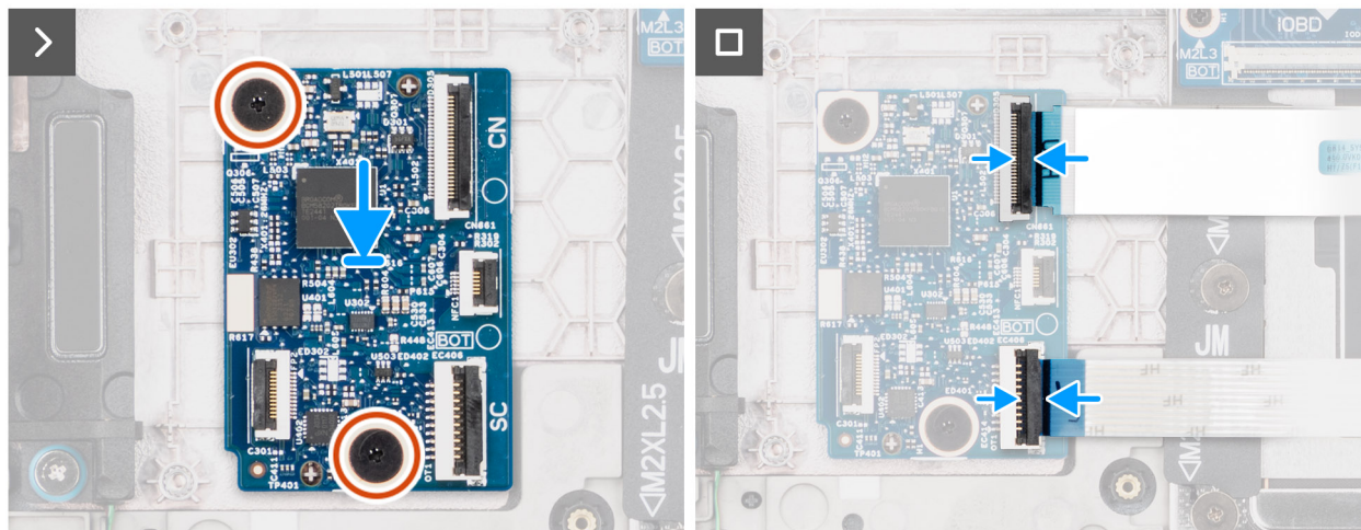
Figure 35. Installing the USH board
