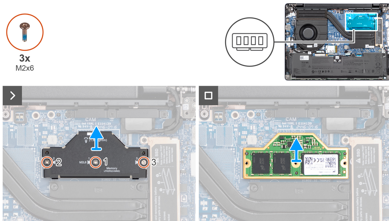
Figure 18. Removing the memory module
