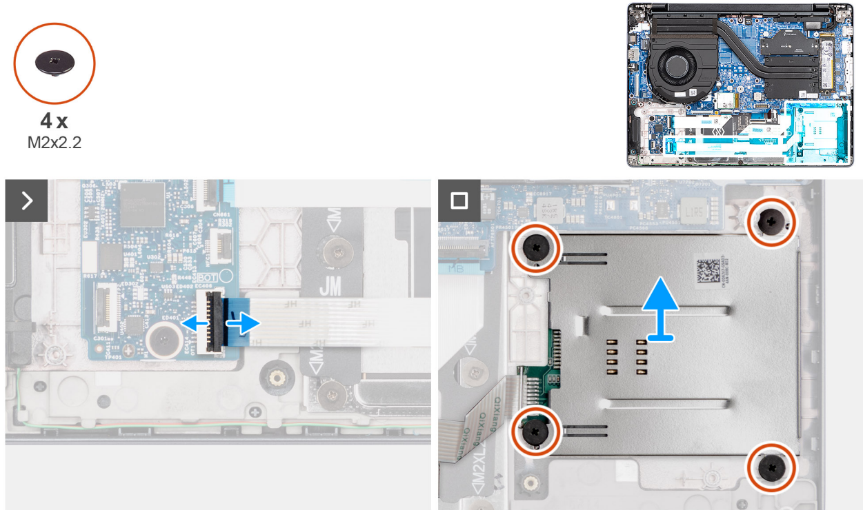
Figure 36. Removing the smart-card reader
