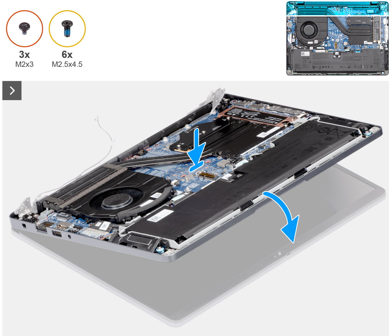
Figure 47. Installing the display assembly
