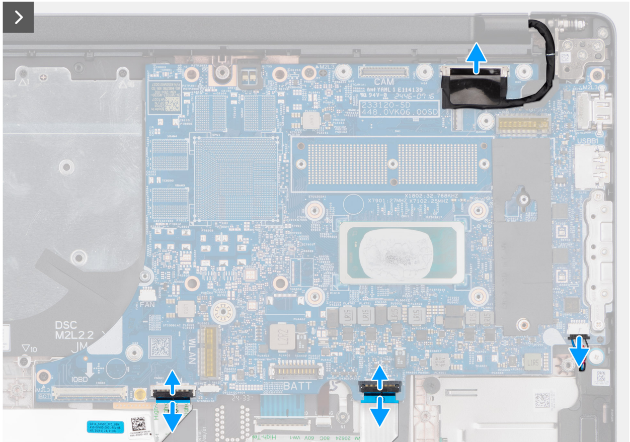
Figure 75. Removing the system board
