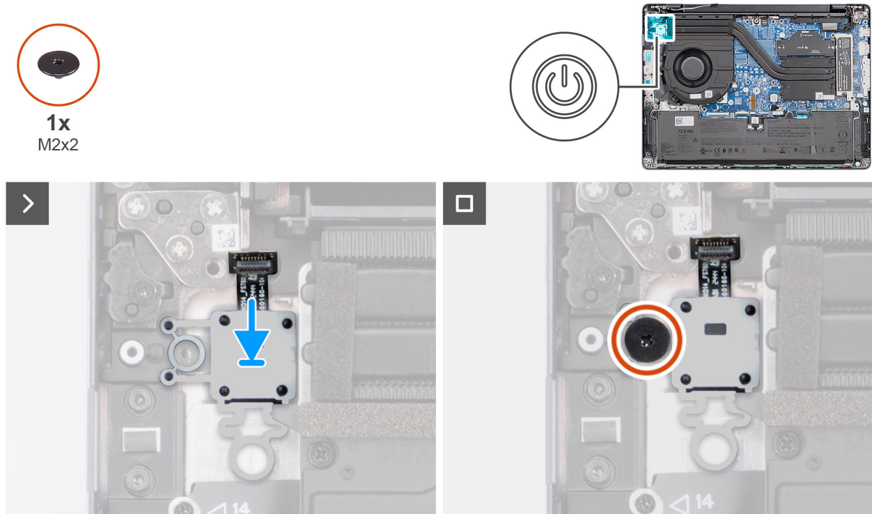
Figure 43. Installing the power button
