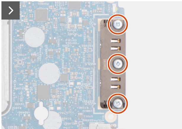
Figure 83. Removing the USB Type-C module
