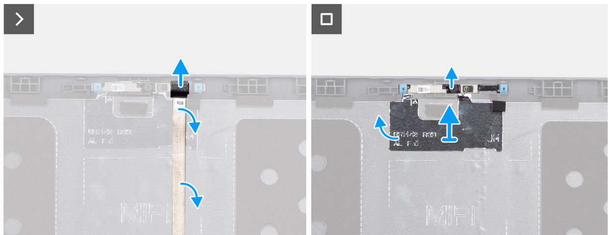
Figure 67. Removing the camera
