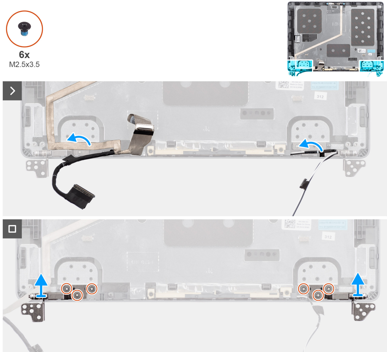
Figure 63. Removing the display hinges
