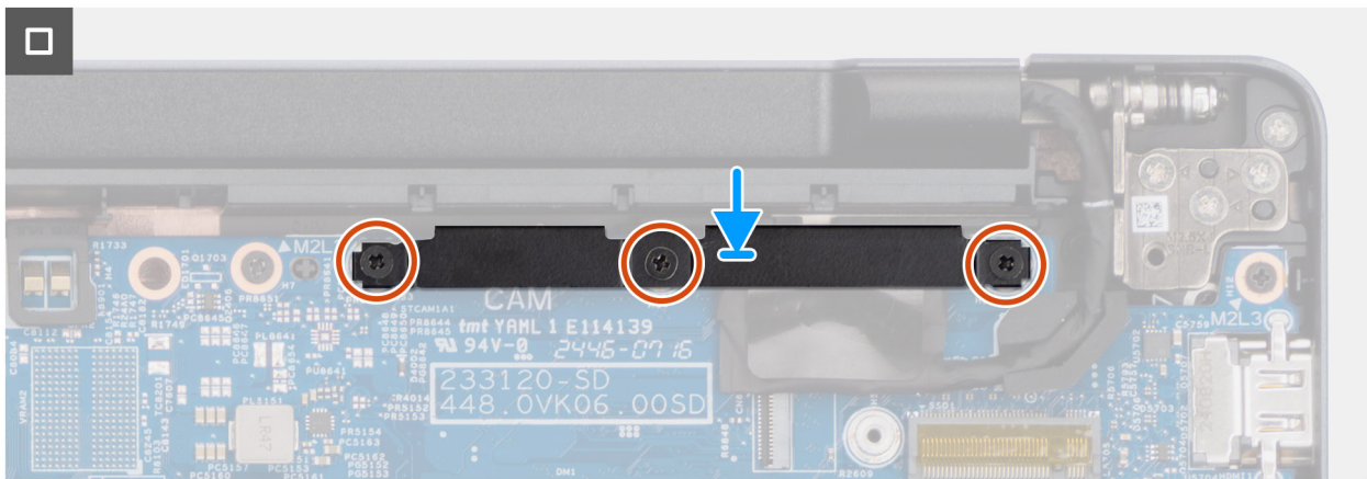
Figure 82. Installing the system board
