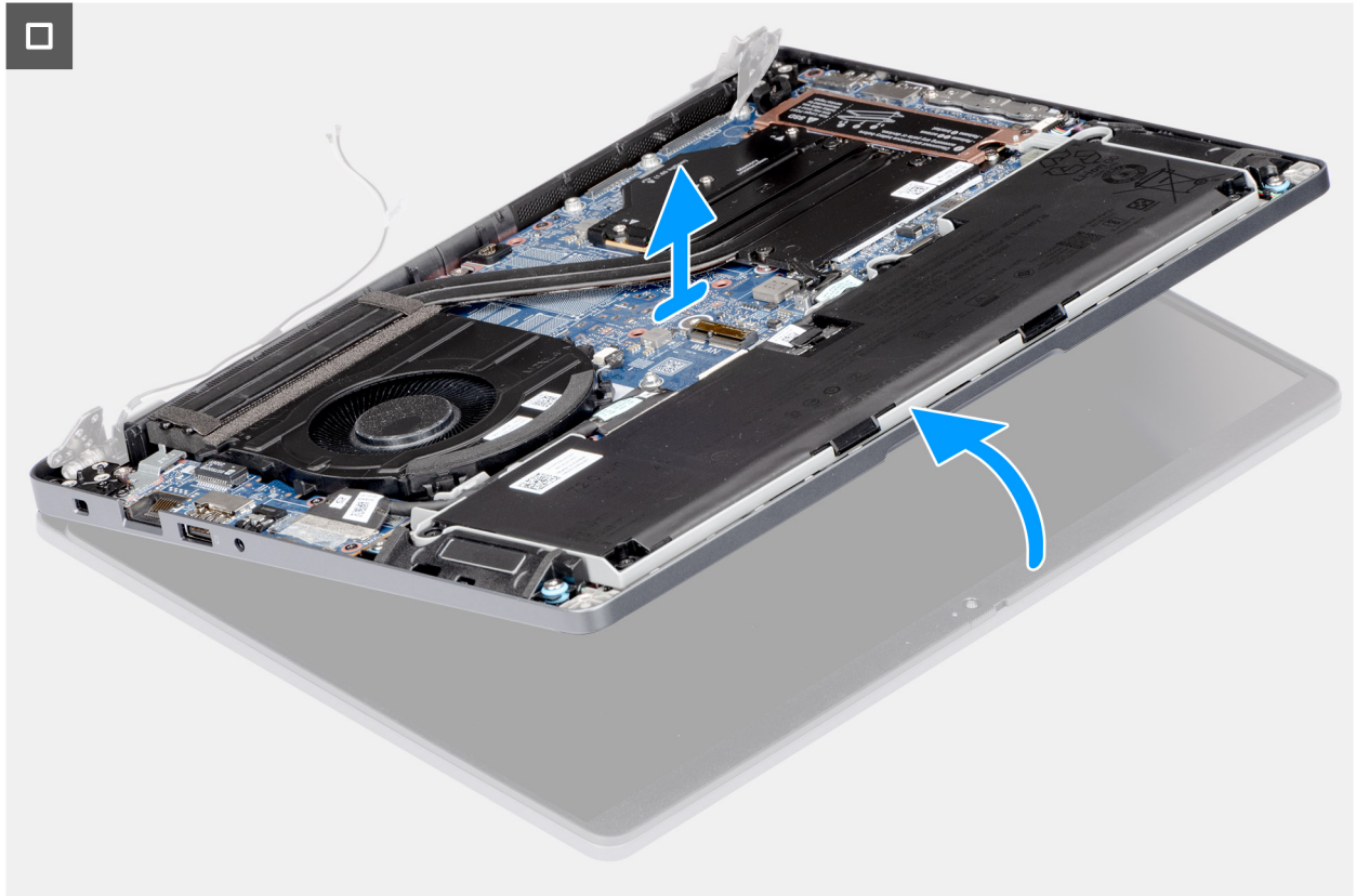
Figure 45. Removing the display assembly
