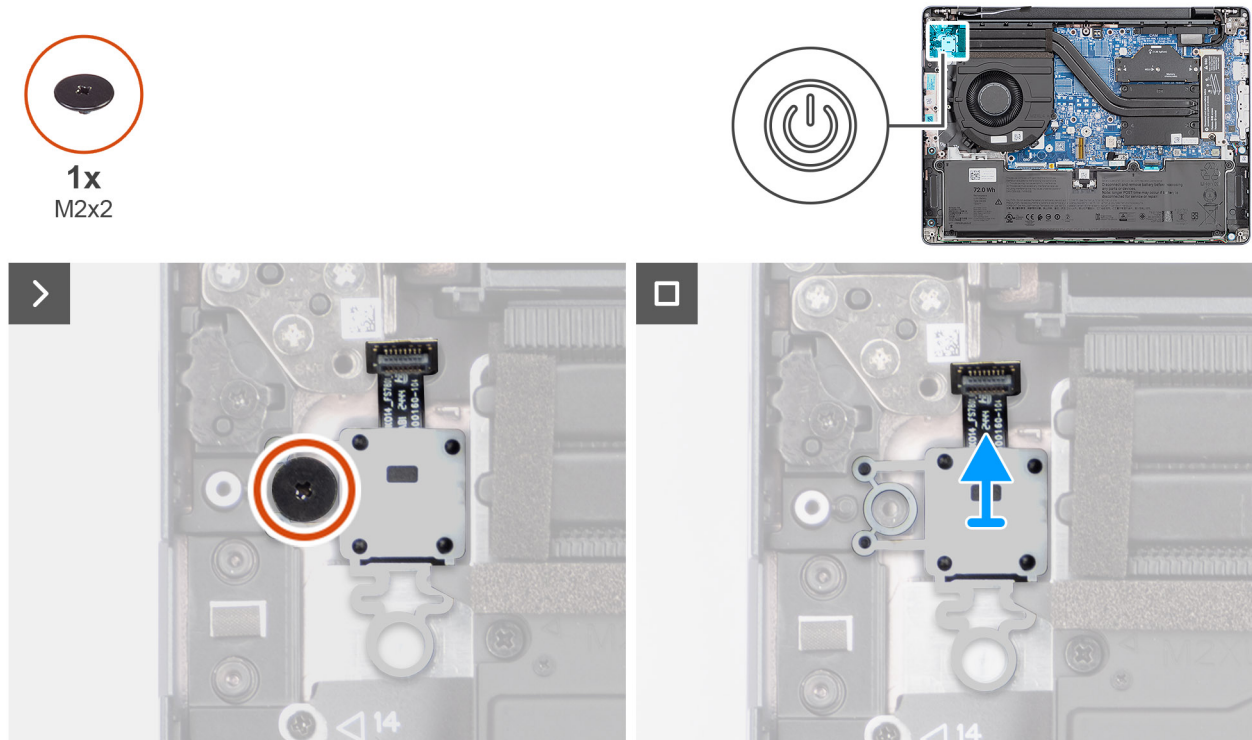
Figure 42. Removing the power button
