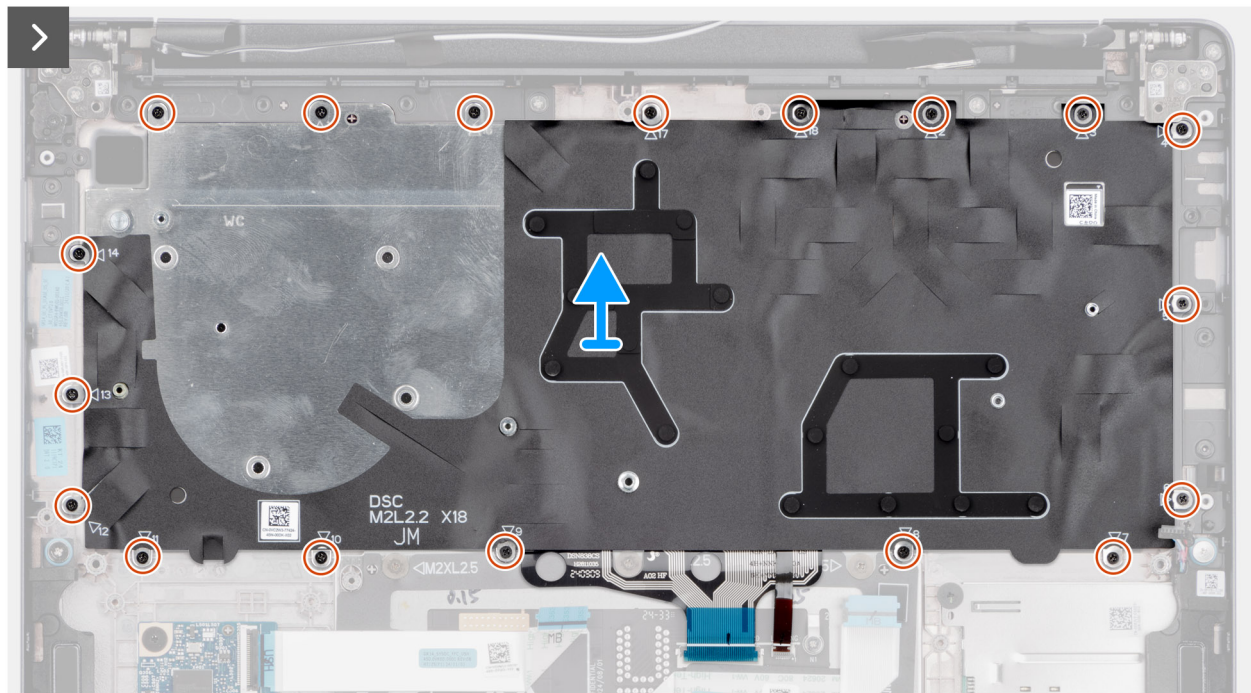
Figure 86. Removing the keyboard
