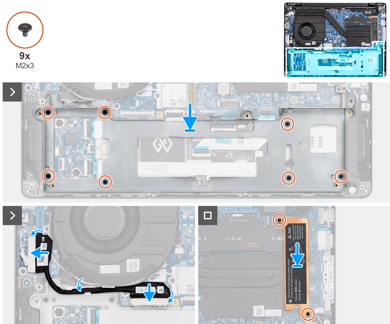
Figure 33. Installing the battery frame
