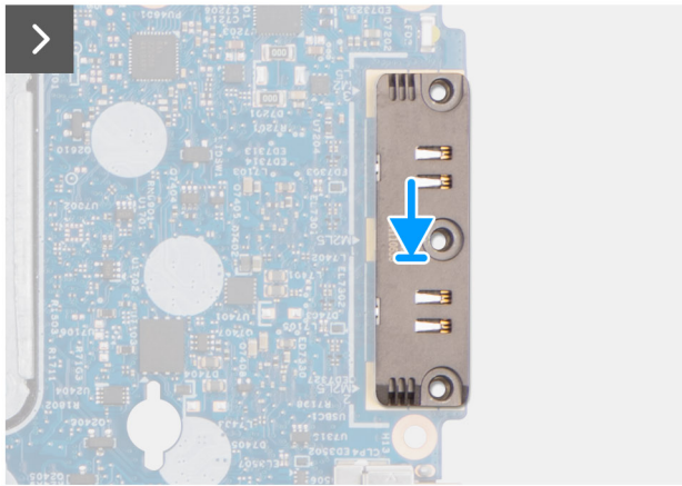
Figure 84. Installing the USB Type-C module
