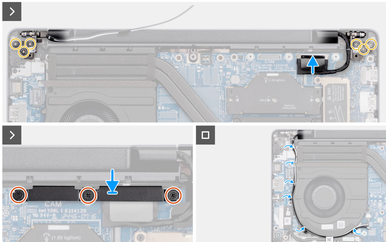
Figure 48. Installing the display assembly
