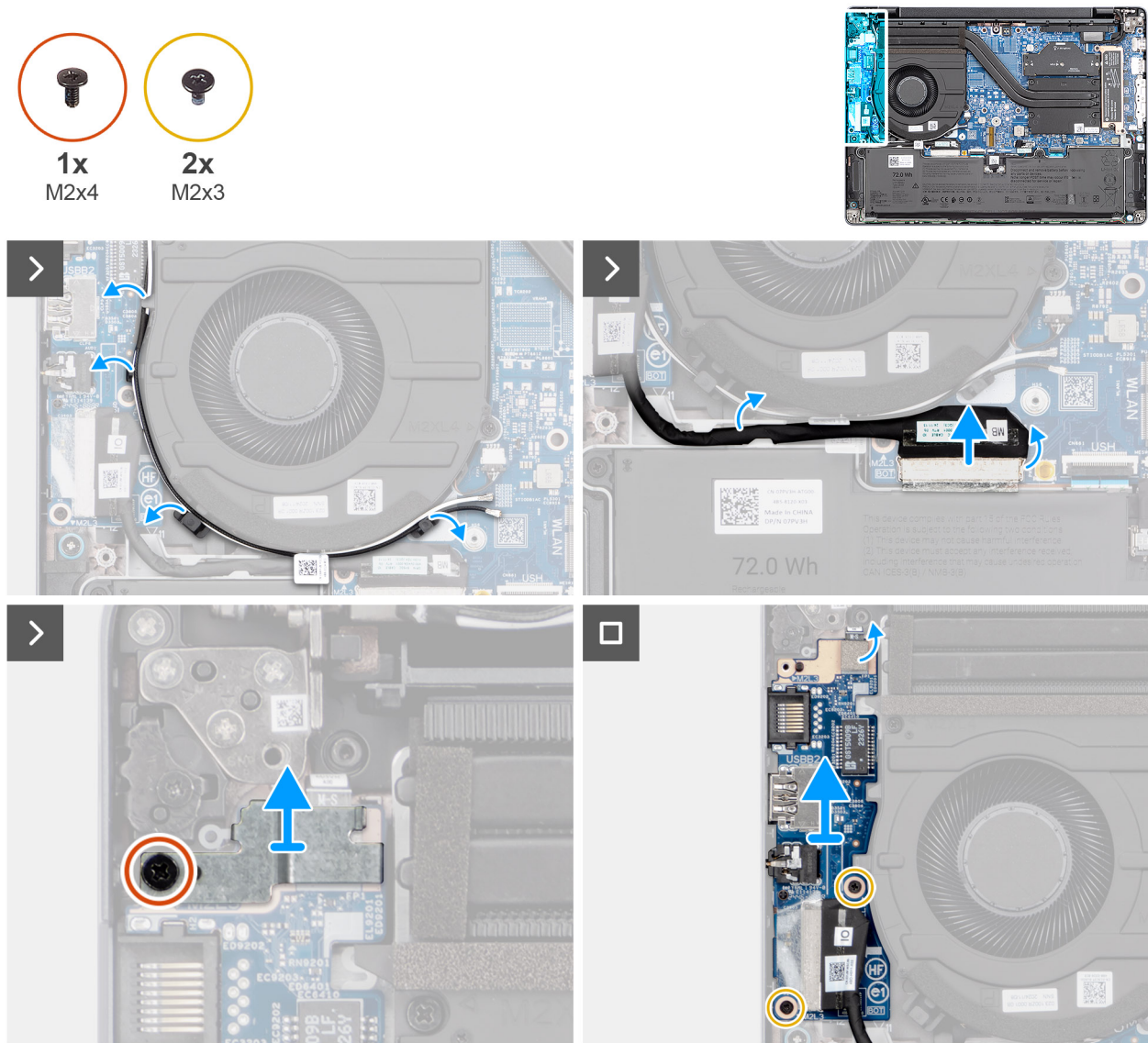
Figure 40. Removing the I/O board
