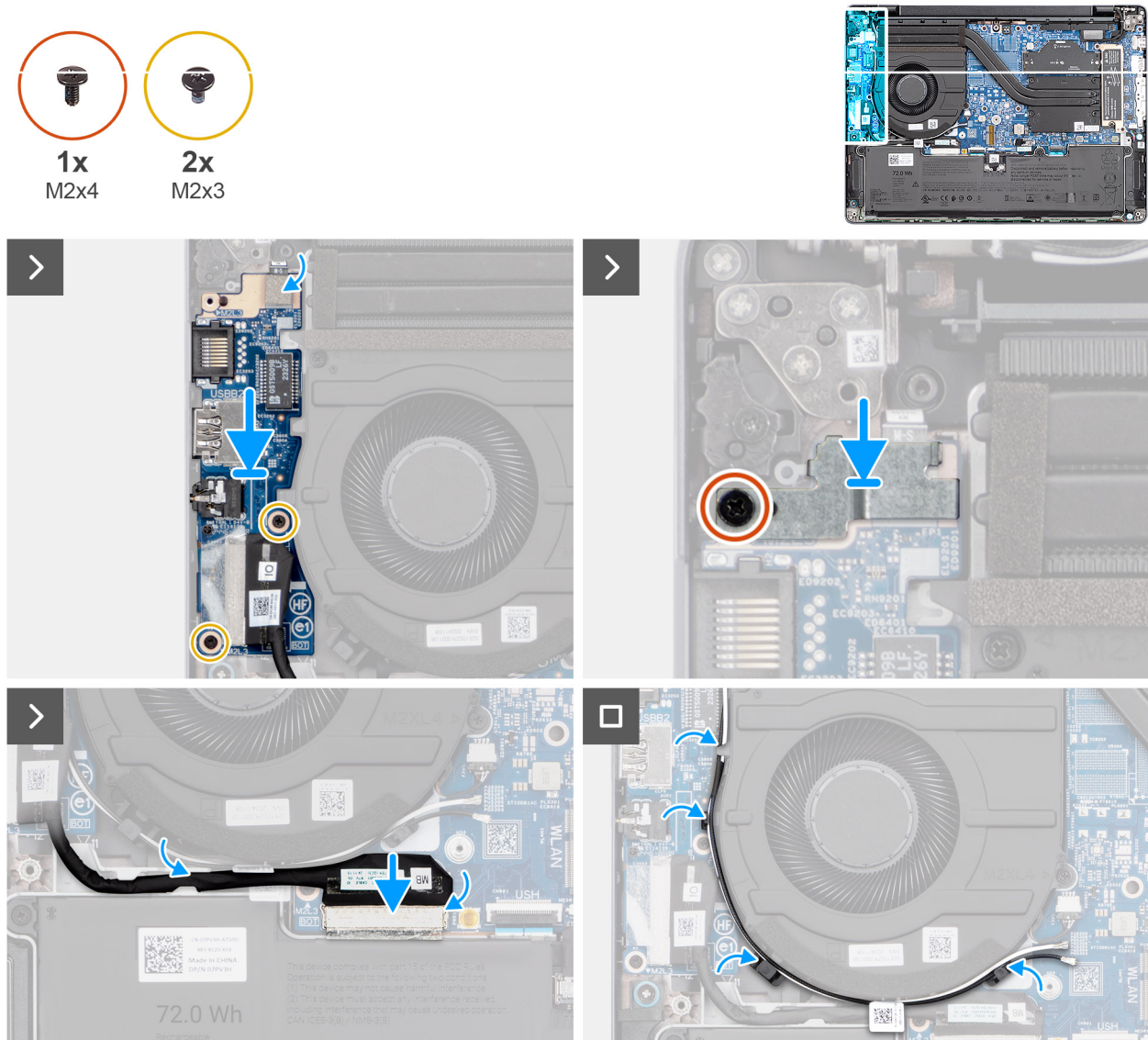
Figure 41. Installing the I/O board
