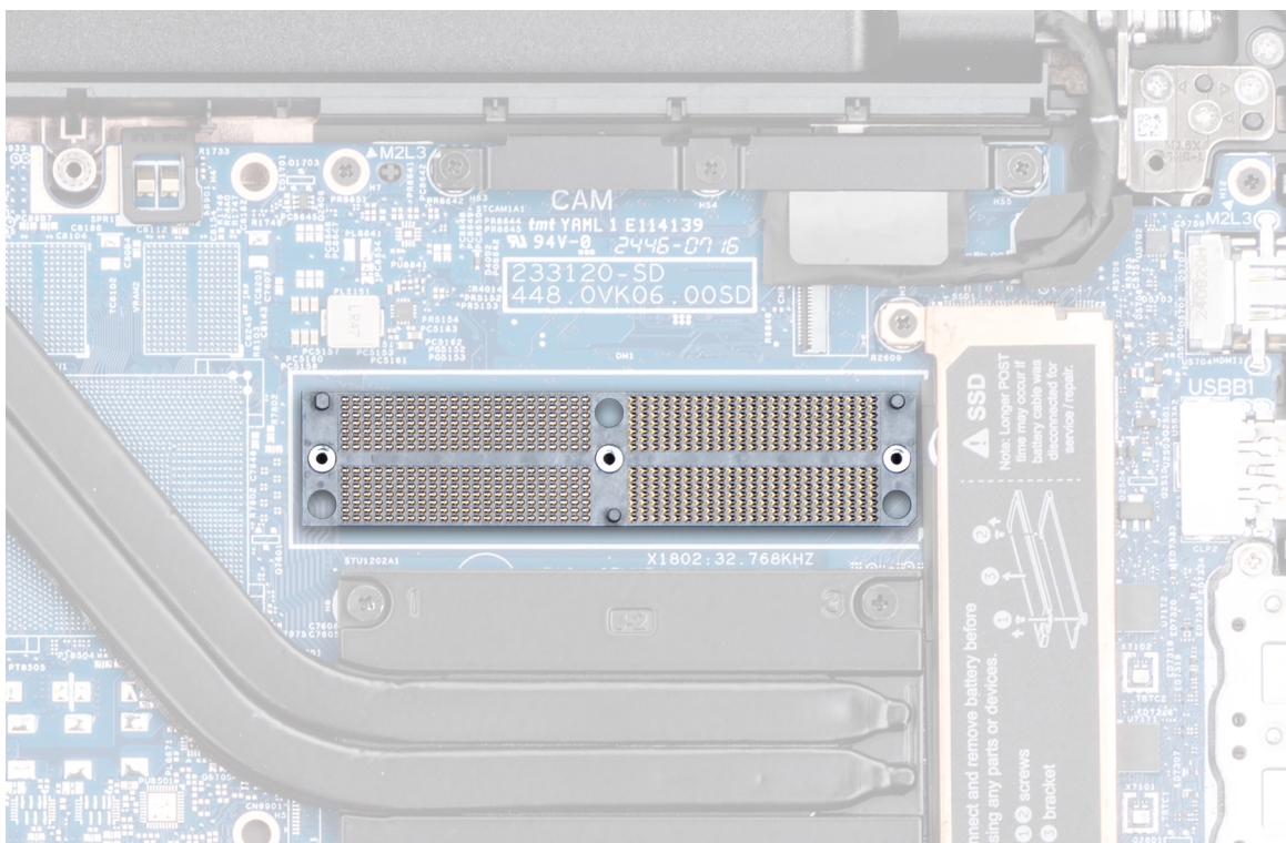
Figure 80. Installing the memory-module connector
