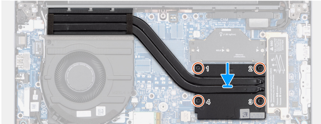
Figure 39. Installing the heat sink
