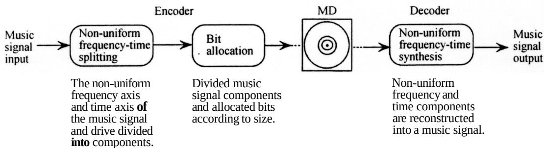
Figure 10.27 ATRAC operation layout.
