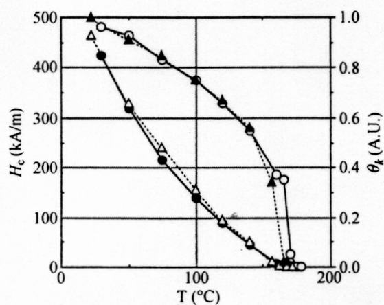
Figure 10.32 Temperature dependence of residual \theta_k and H_c .
