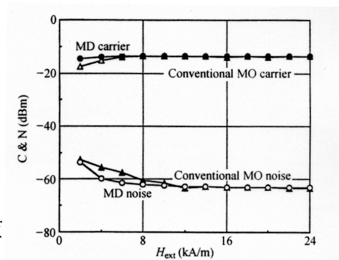
Figure 10.35 Bias field dependence of carrier and noise v = 1.22\text{m/s} , laser power = 4.55 mW, mark length = 0.85 \mu\text{m} .
