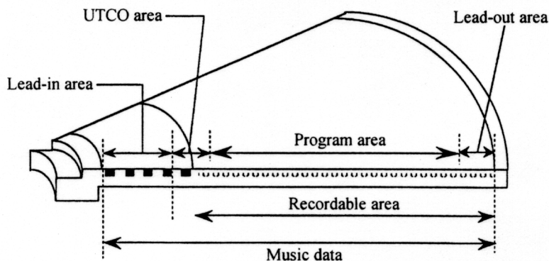
Figure 10.25 Cross section of a recordable MiniDisc.
