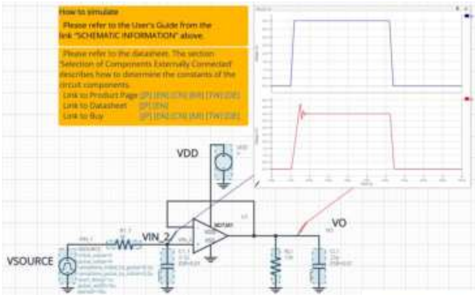
Figure 1. Simulation Schematic
