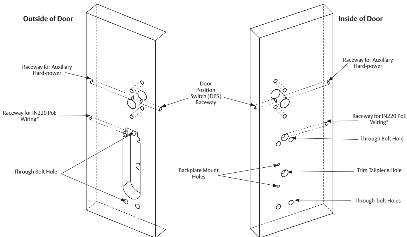
Figure 5-1B Wood Door Preparation
