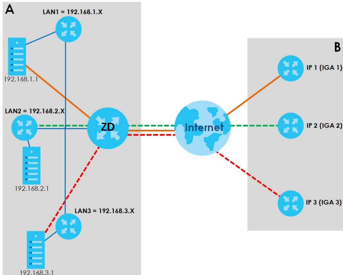
Figure 146 NAT Application With IP Alias
