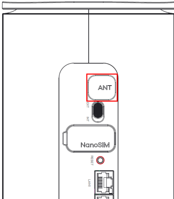
Figure 27 NR5307 External Antenna Connector
