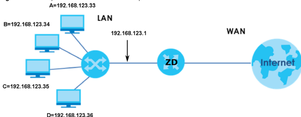
Figure 137 Multiple Servers Behind NAT Example
