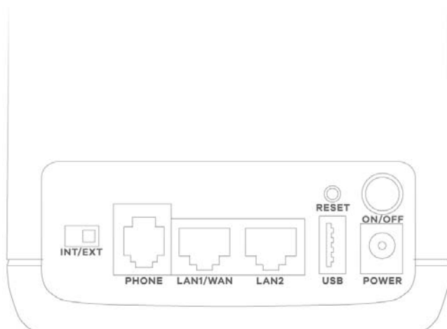
Figure 28 NR5101 Ports and Buttons
