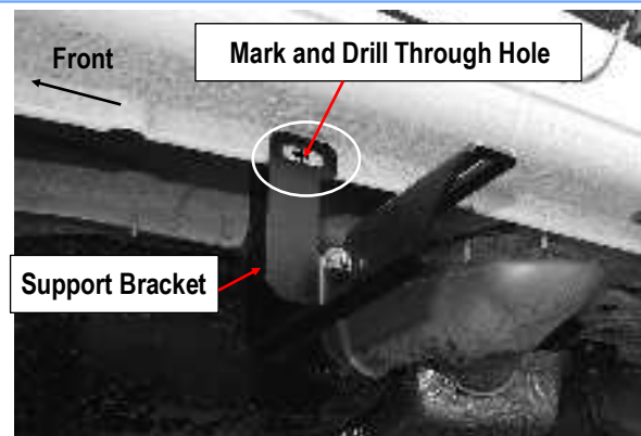
(Fig 11) Mark and Drill Through Holes on Pinch Weld
