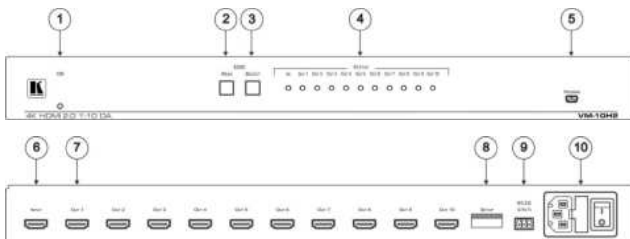
Figure 1: VM-10H2 4K HDMI 2.0 1:10 DA Front Panel
