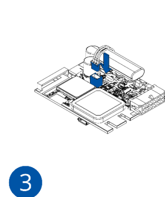
Figure 5 Battery connection
