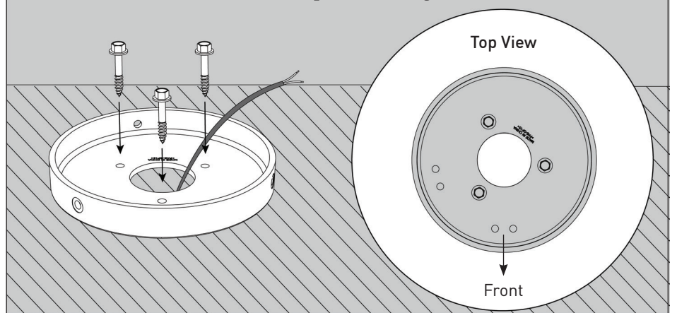
Fig. 2 Hardscape Mounting
