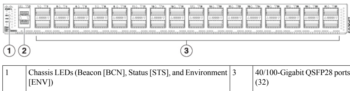
Figure 1: Port Side View of the Cisco Nexus 9332C Switch
