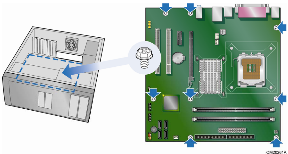
Figure 5. Desktop Board D945GCNL Mounting Screw Hole Locations
