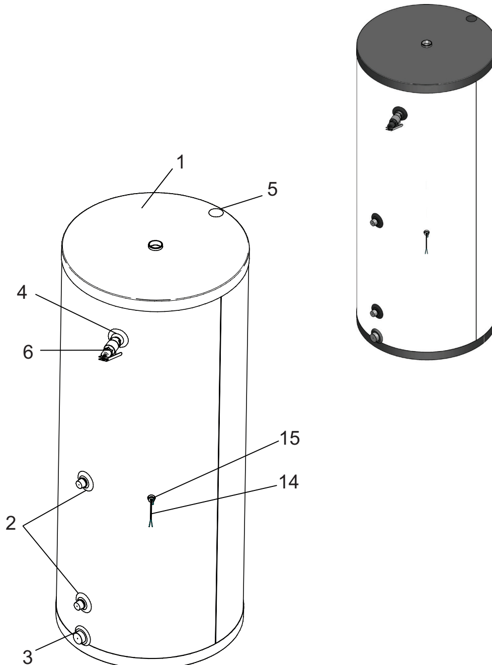
STAINLESS STEEL INDIRECT TANK (SIT_SIT DW)
