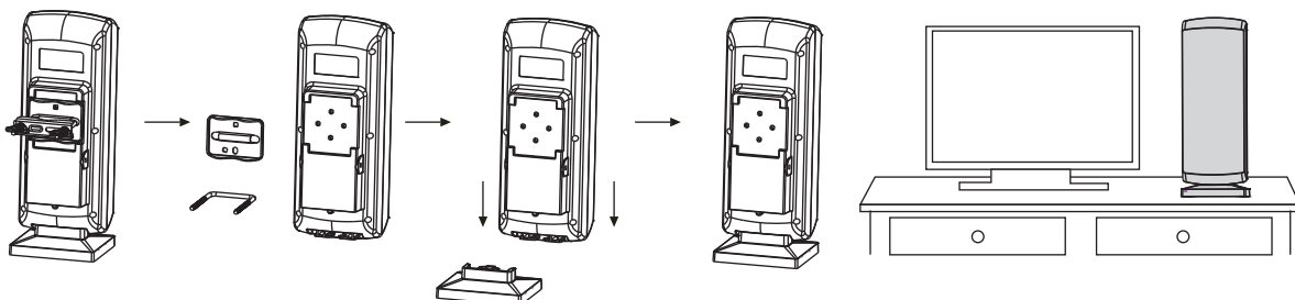
(Fig.4) Indoor installation (optional)
