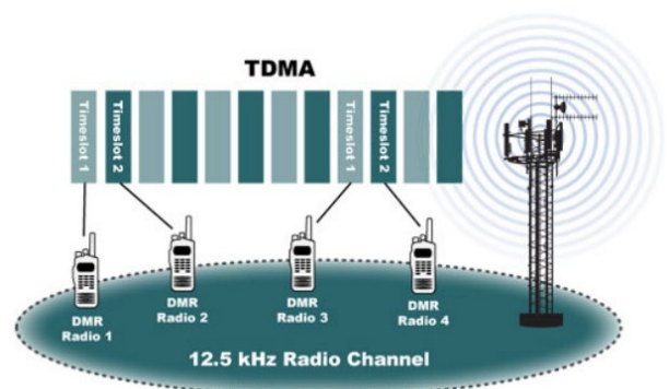
Two Timeslot TDMA structure of DMR Radios
