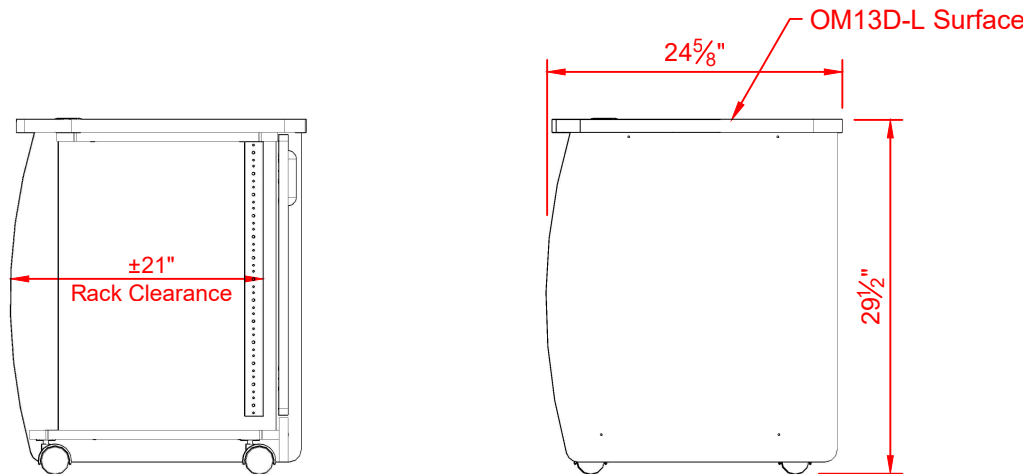
CUTAWAY VIEW
