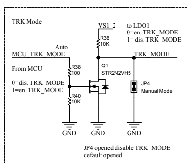
Figure 3. AEK-POW-LDOV02X circuit schematic (3 of 3)
