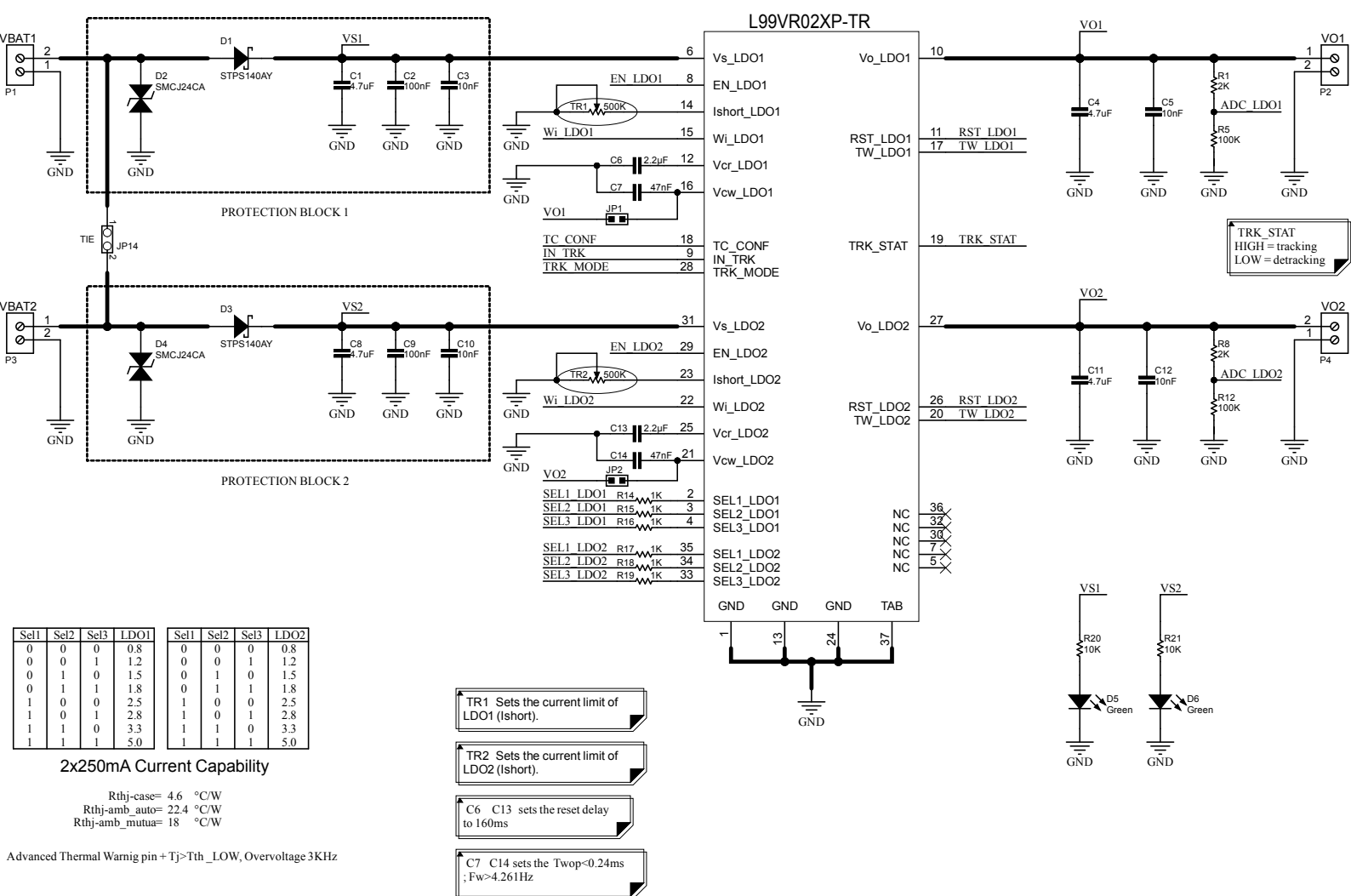
Figure 1. AEK-POW-LDOV02X circuit schematic (1 of 3)
