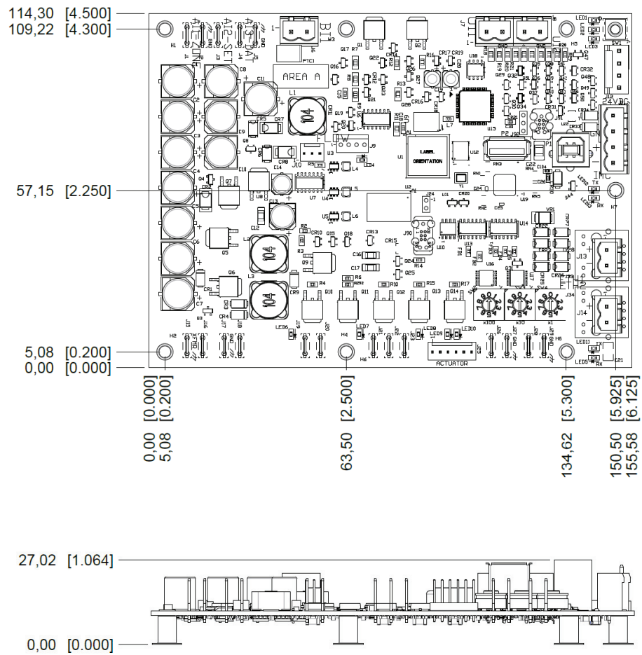
Figure 1. Controller dimension
