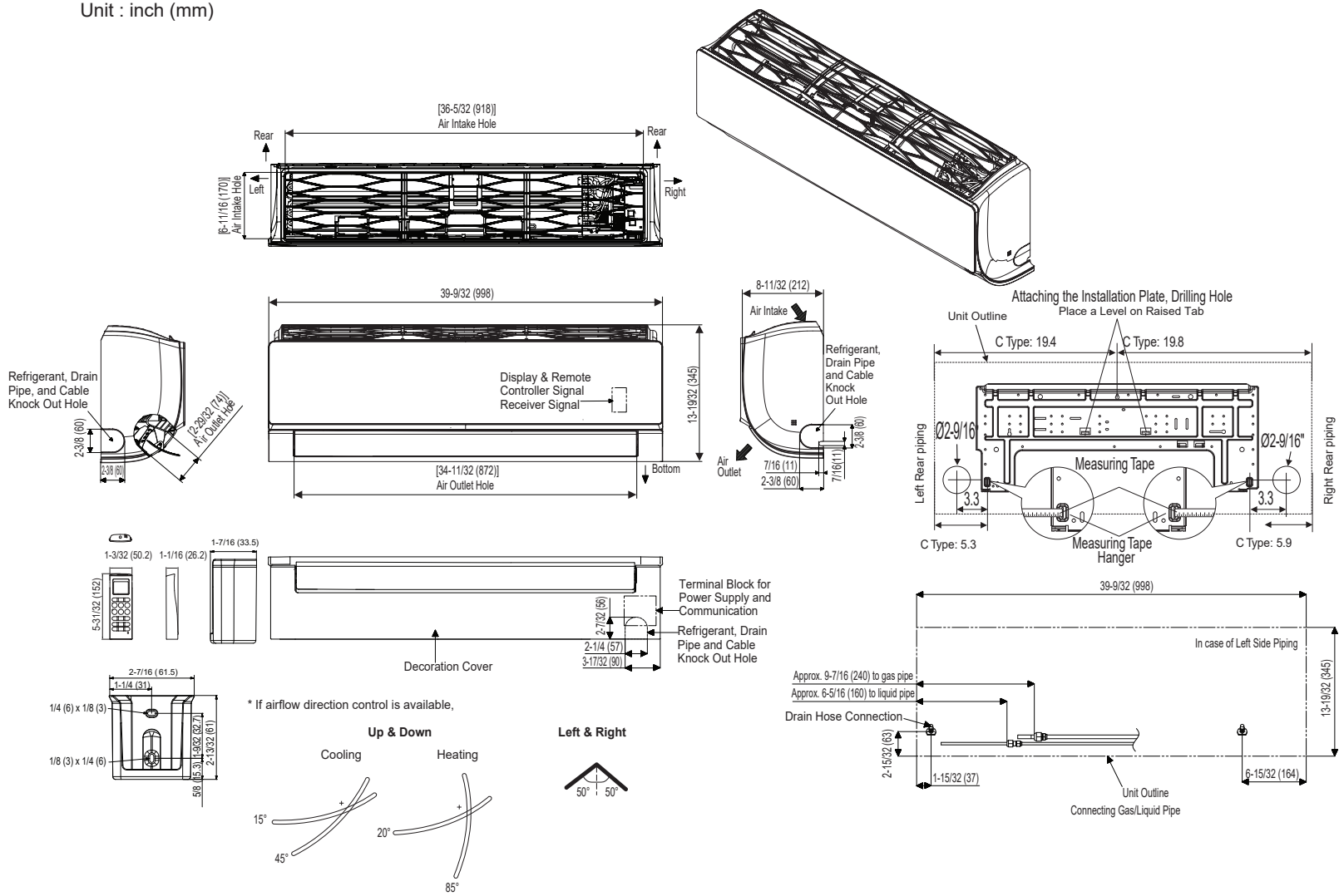
Figure 3: LAN180HSV5 Dimensions.
