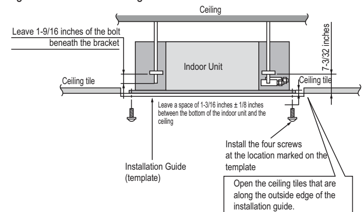
Figure 198: Installation Diagram.
