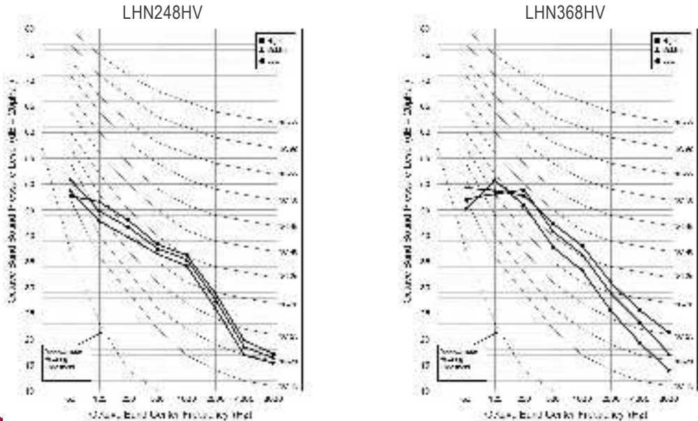
Figure 156: Sound Pressure Level Diagrams.
