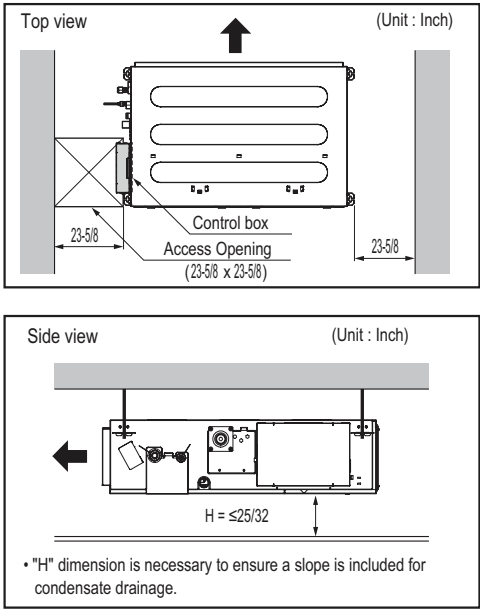
Figure 128:General Installation Guidelines.
