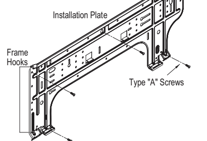
Figure 73: Installation Plate—Side View.
