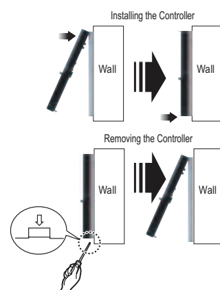
Figure 147: Installing / Removing the Controller.
