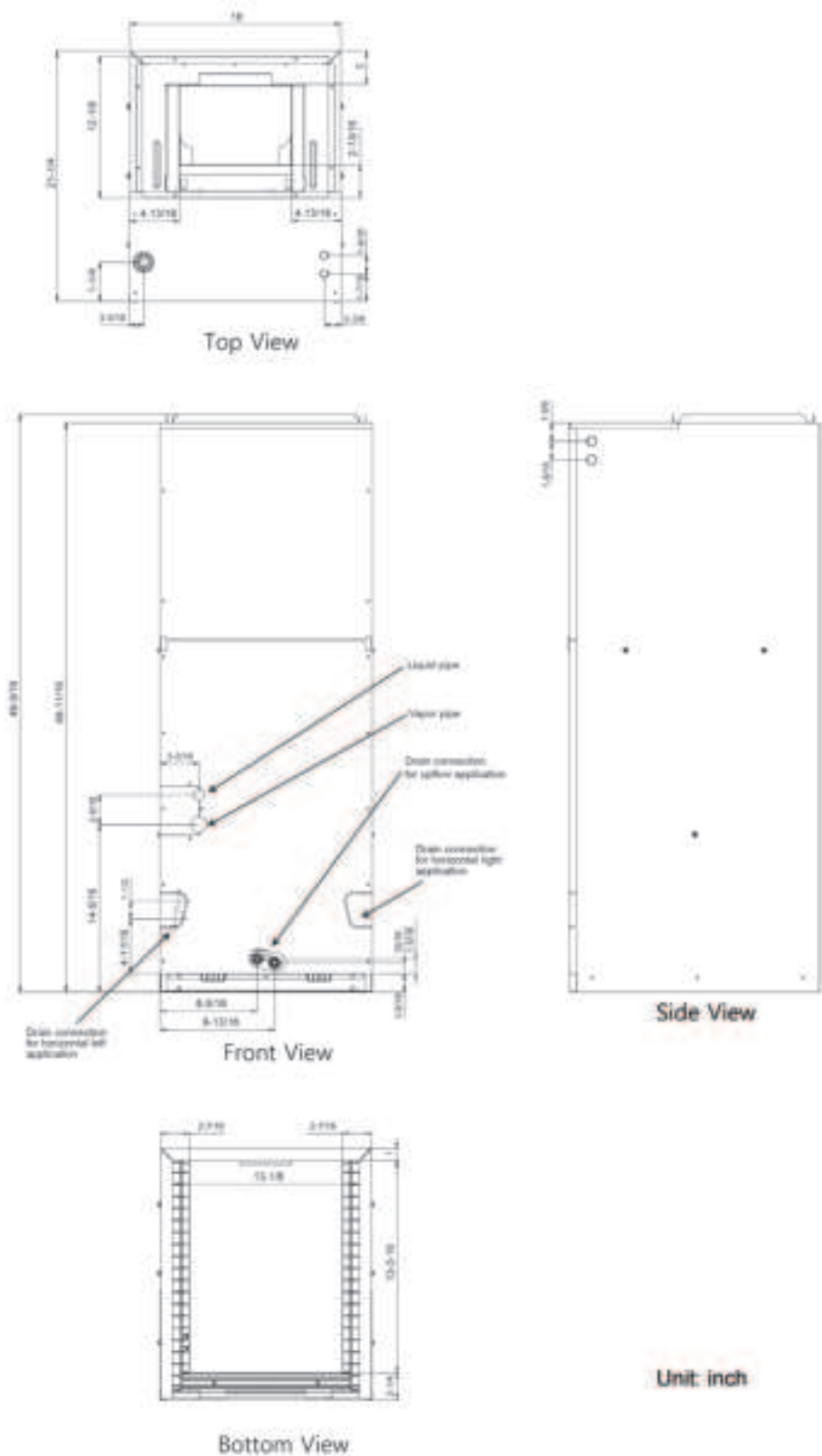
Figure 216: Four-way Vertical Air Handling Unit Dimensions.
