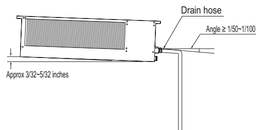
Figure 138: Checking the Drain Pump.
