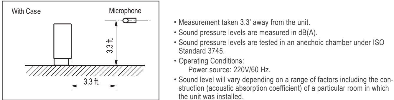
Figure 218: Sound Pressure Level Measurement Location.
