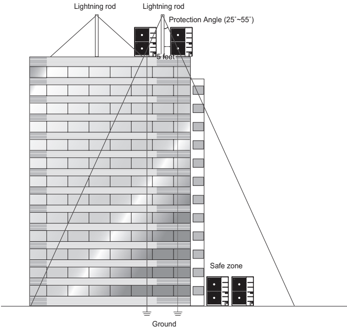
Figure 251: Lightening Protection Diagram.
