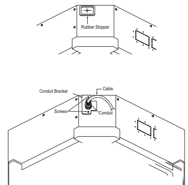
Figure 205: Using a Conduit.
