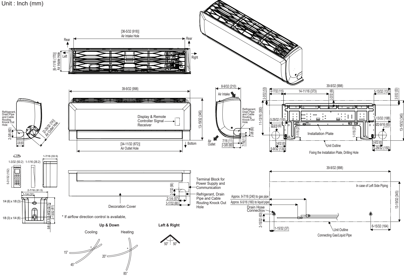
Figure 62: LSN180HSV5 and LMN249HVT Dimensions.
