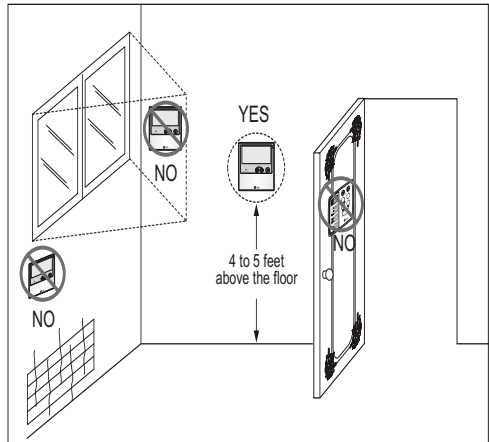
Figure 89:Proper Location for the Wired Controller.
