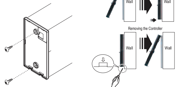
Figure 245: Attaching the Wall Plate.
