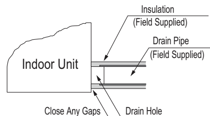
Figure 135: Drain Connection.
