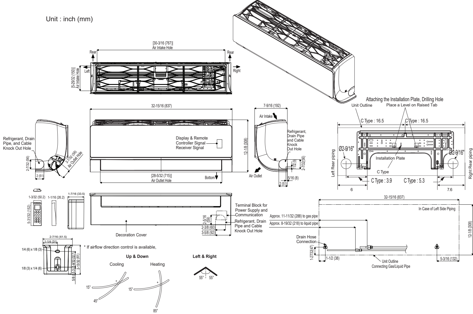
Figure 2: LAN090HSV5 and LAN120HSV5 Dimensions.
