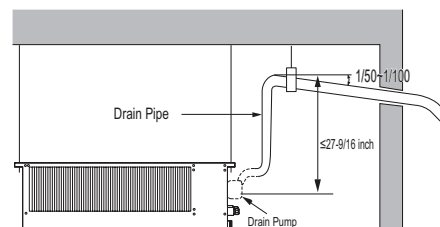
Figure 136: Indoor Unit Using Drain Pump.
