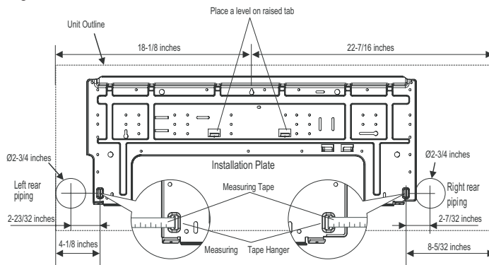
Figure 75: Installation Plate for LSN180HSV5 and LMN249HVT Units.
