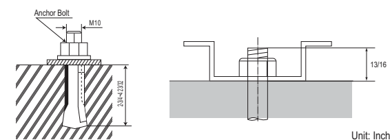
Figure 250: Close up of Bolt Attachment.
