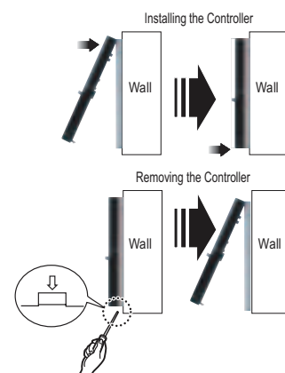
Figure 58: Installing/Removing the Controller.
