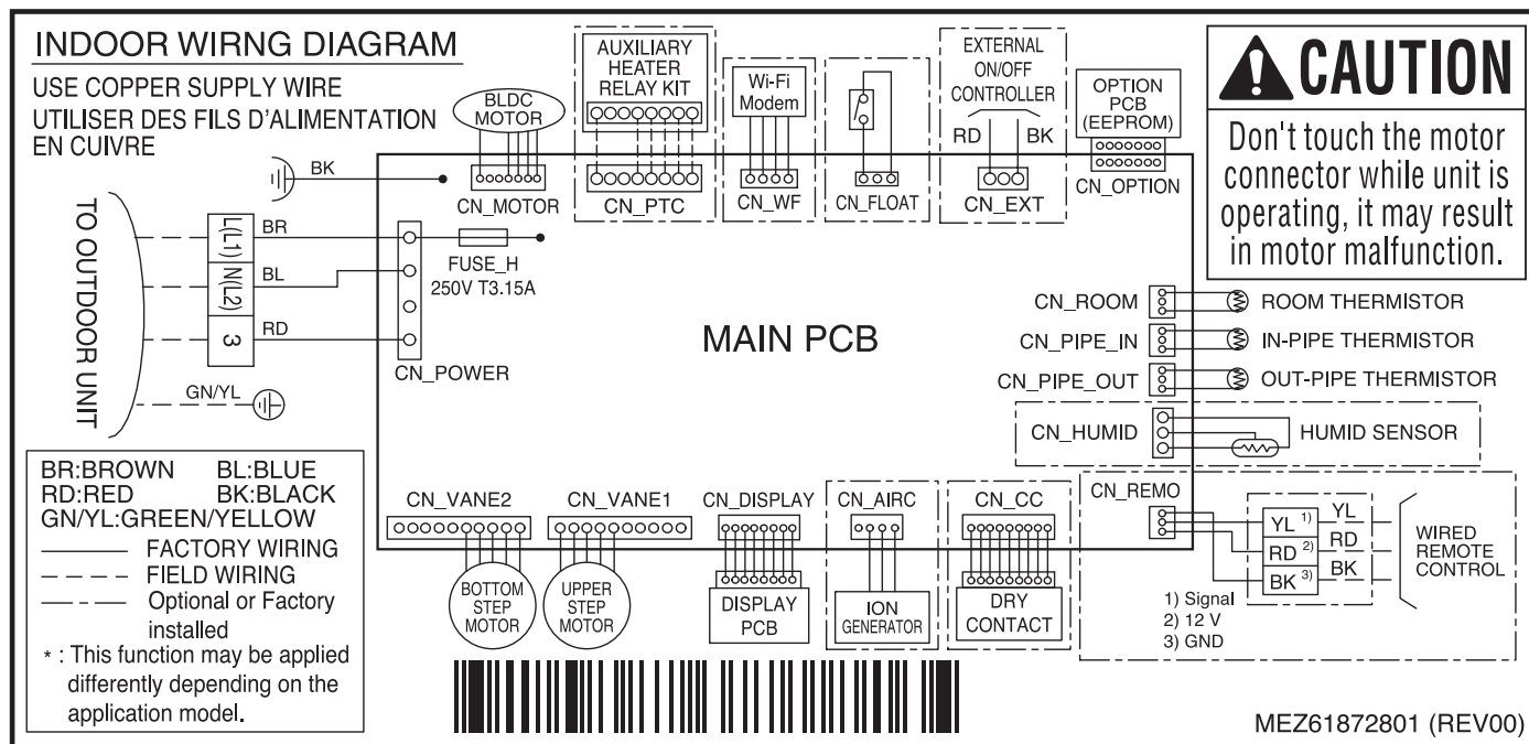
Figure 103: Multi F Low Wall Console LQN090HV4, LQN120HV4, and LMQN150HV Indoor Units Wiring Diagram.
