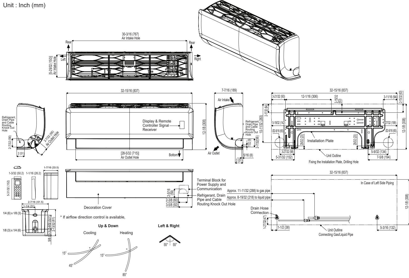
Figure 61: LMN079HVT, LSN090HSV5, LSN120HSV5, and LMN159HVT Dimensions.
