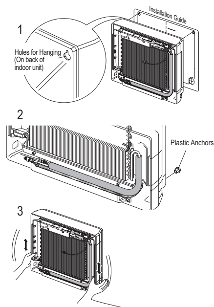
Figure 45: Hanging the Indoor Unit Frame.
