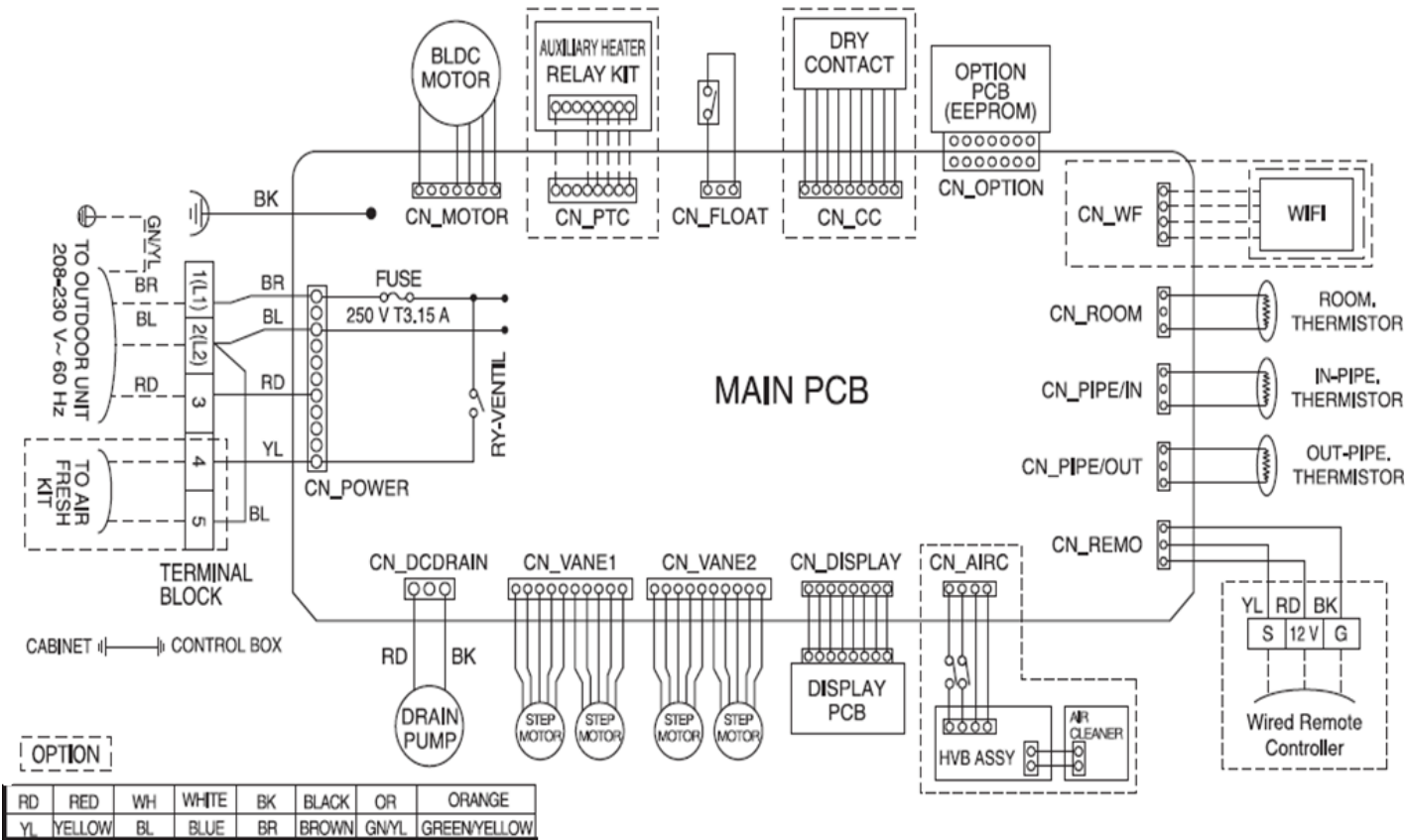
Figure 192:Multi F Four-Way Ceiling-Cassette Indoor Unit Wiring Diagram.
