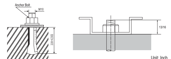
Figure 250: Close up of Bolt Attachment.
