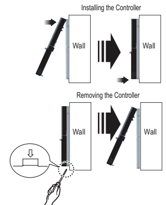
Figure 147: Installing / Removing the Controller.
