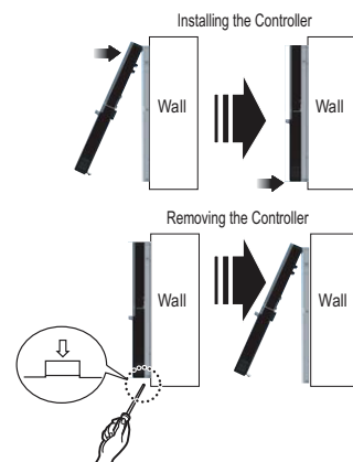
Figure 93: Installing / Removing the Controller.
