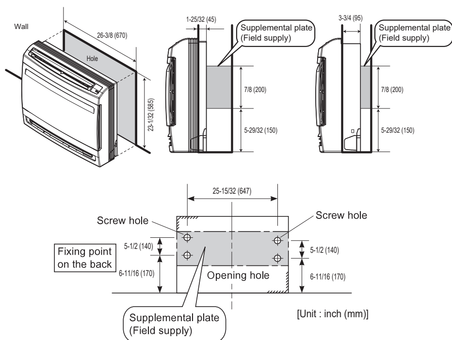
Figure 107: Recessed Installation.
