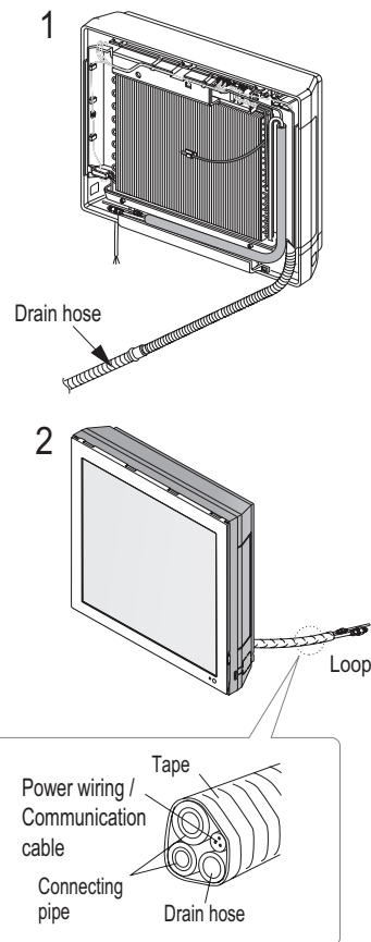
Figure 43: Preparing the Refrigerant / Drain Connections.
