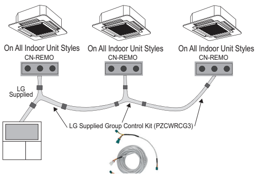
Figure 275:Example of Indoor Unit Group to Zone Controller Connections (CN-REMO).
