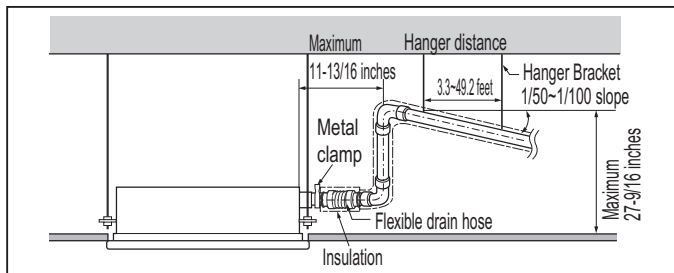
Figure 165: Drain Piping Installation Dimensions.
