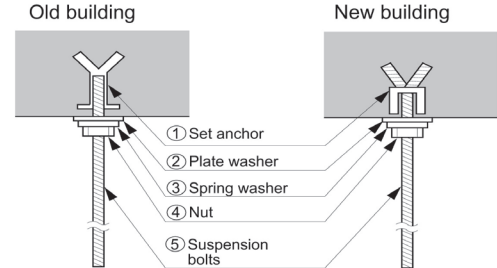
Figure 133:Console Bolt Options.
