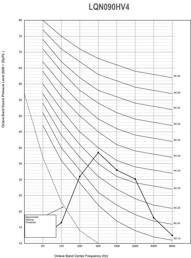
Figure 98: LQN090HV4 and LQN120HV4 Sound Pressure Level Diagrams.
