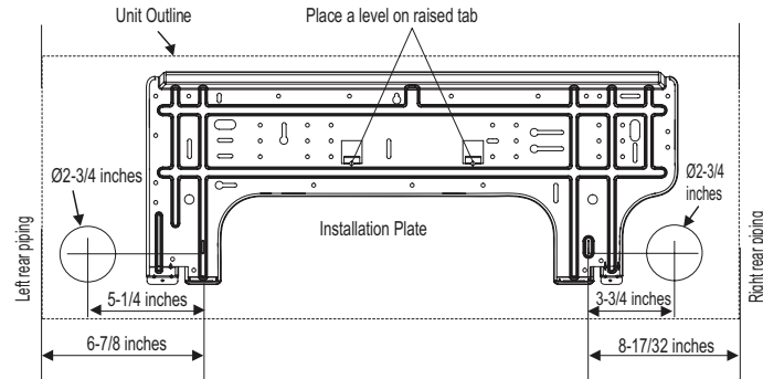
Figure 11: Installation Plate for LAN090HSV5 and LAN120HSV5 Units.
