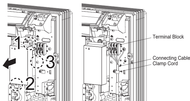
Figure 110: Connecting Power Wiring / Communications Cable.
