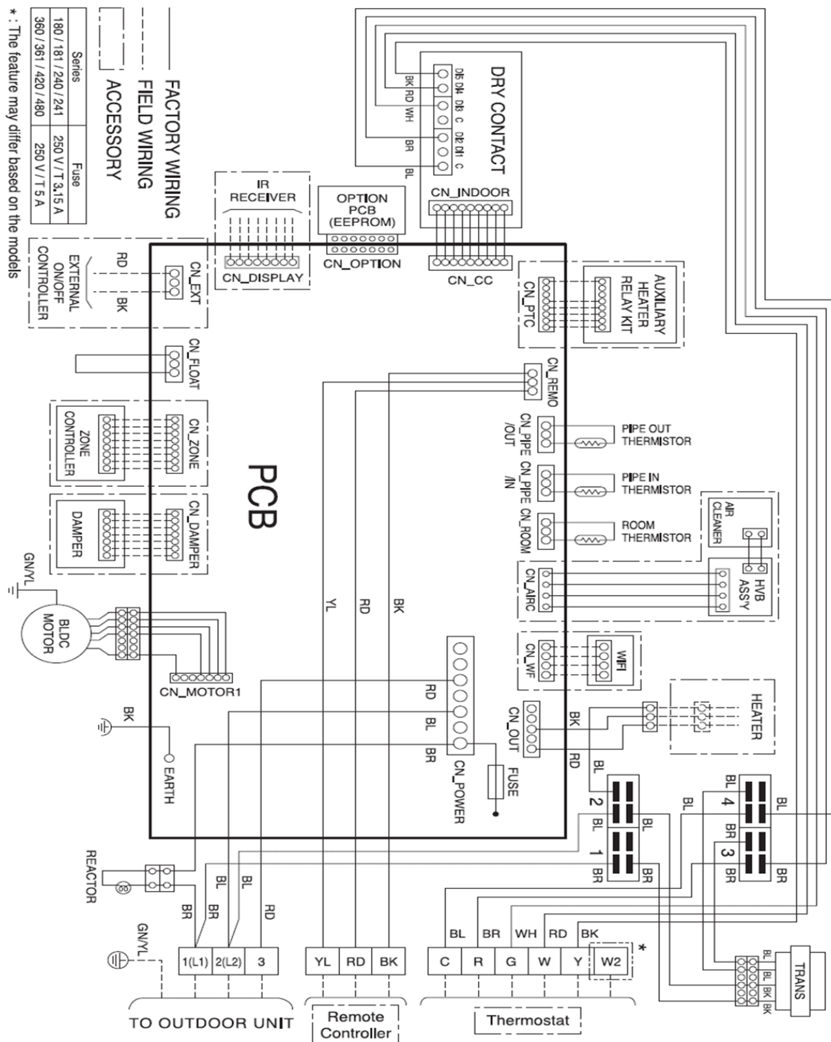
Figure 222: Four-way Vertical-Horizontal Air-Handling Indoor Unit Wiring Diagram.
