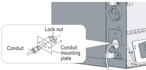
Figure 142: Exterior View of Conduit Installation.
