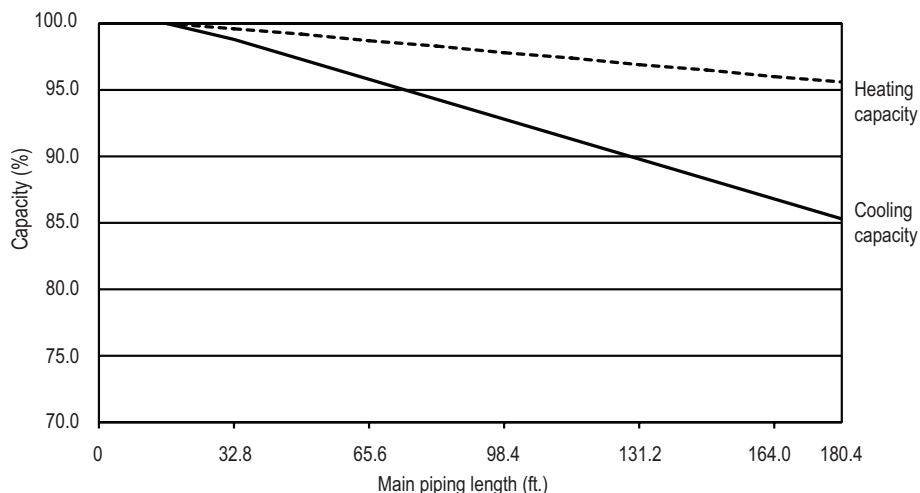
Figure 247: Multi F MAX / Multi F MAX with LGRED Outdoor Unit to Branch Distribution Unit Refrigerant Line Length Derate Chart.
