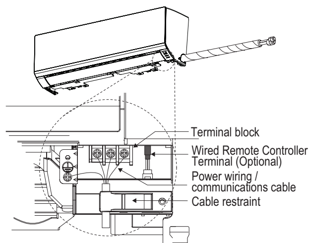
Figure 83: Connecting Power Wiring / Communications Cable.
