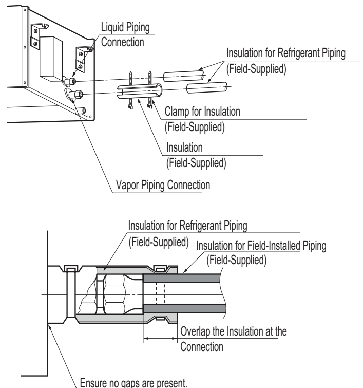
Figure 168: Insulating the Piping.
