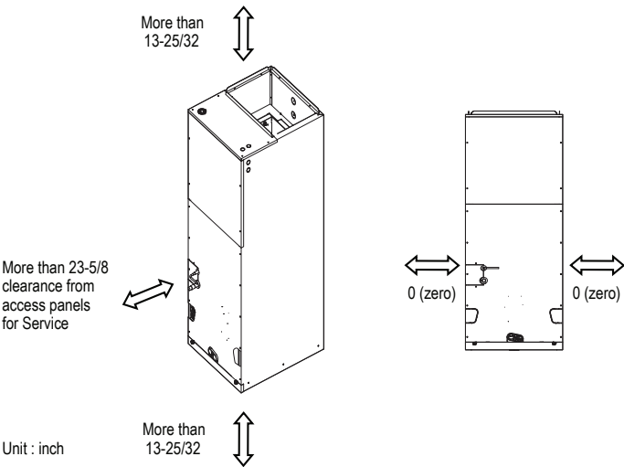
Figure 223:Clearance Requirements.
