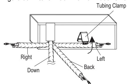
Figure 80: Exterior Back View of Indoor Unit.
