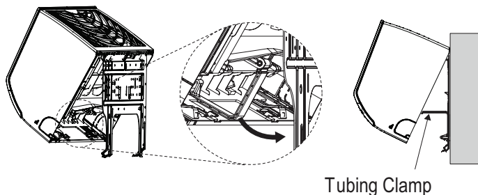
Figure 78: Accessing the Back of the Indoor Unit.
