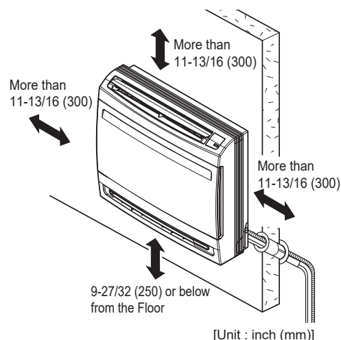
Figure 104: Minimum Clearance Requirements.
