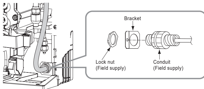
Figure 112: Securing Wiring to Unit.
