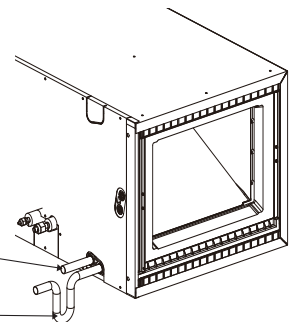
Figure 236: Horizontal Primary and Secondary Drain Layout.
