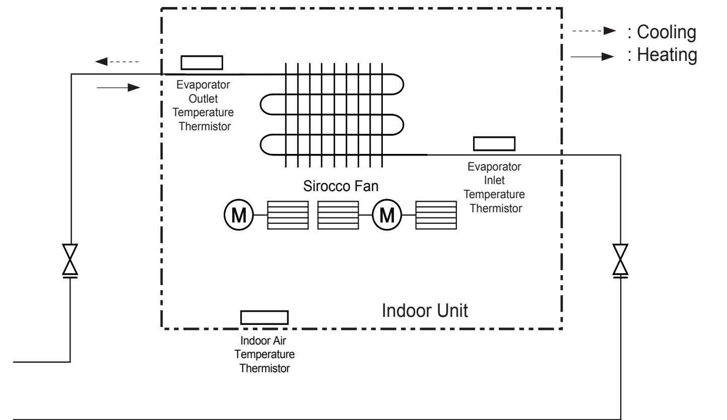
Figure 125:LDN127HV4 and LDN187HV4 Refrigerant Flow Diagram.
