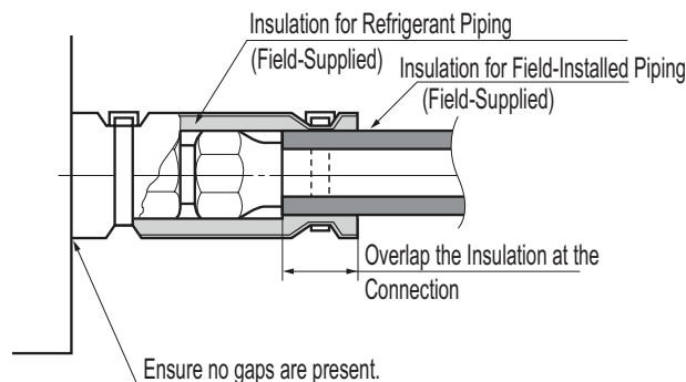
Figure 202: Insulating the Piping.
