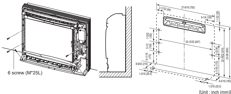
Figure 105: Floor Installation
