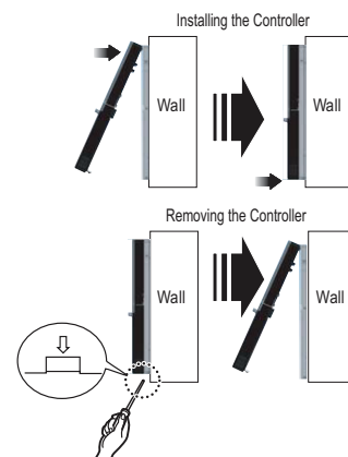
Figure 119: Installing / Removing the Controller.
