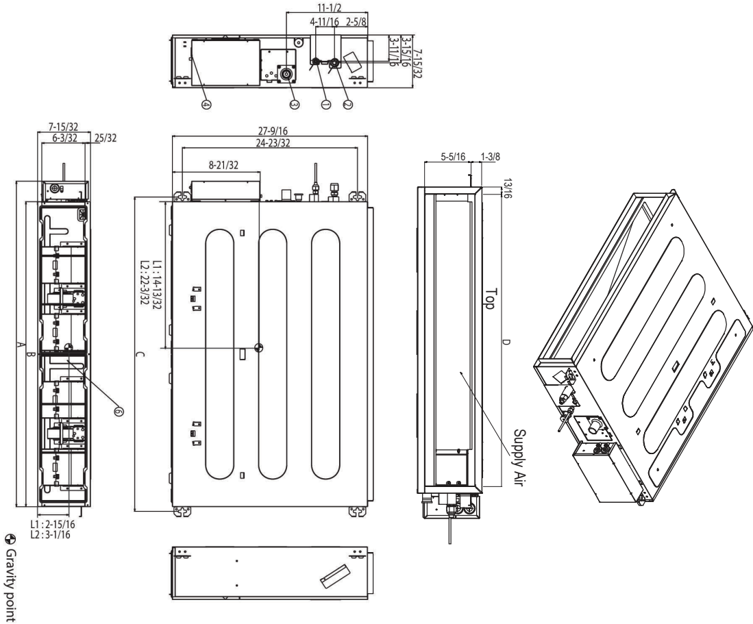
Figure 121:LDN097HV4, LDN127HV4, and LDN187HV4 Dimensions.
