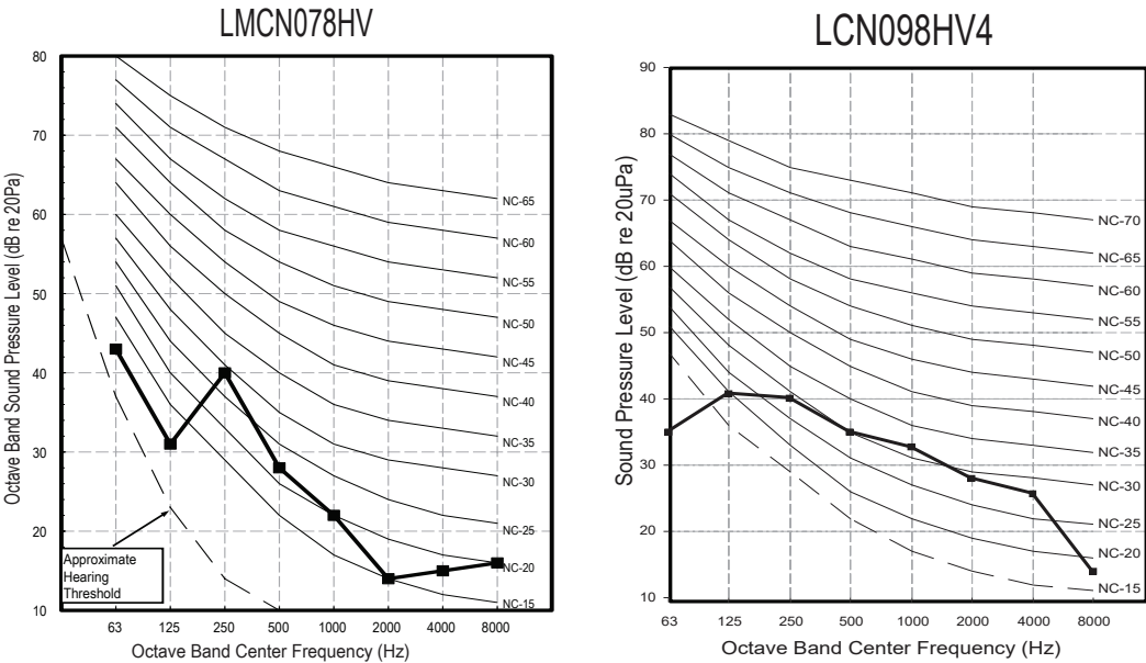
Figure 185:LMCN078HV and LCN098HV4 Sound Pressure Level Diagrams.
