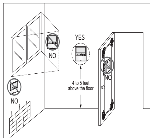
Figure 116:Proper Location for the Wired Controller.
