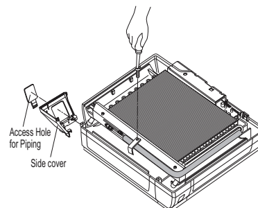
Figure 41: Removing the Piping and Side Covers.
