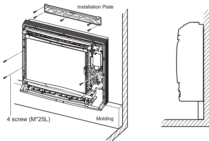
Figure 106: Wall Installation.
