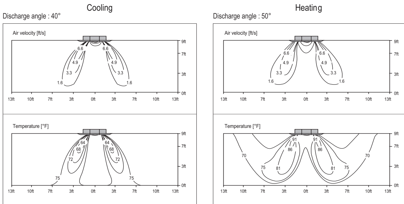
Figure 190: LCN188HV4 Air Velocity and Temperature Distribution Charts.
