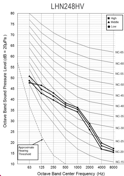
Figure 156: Sound Pressure Level Diagrams.
