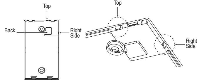
Figure 211: Attaching the Wall Plate.
