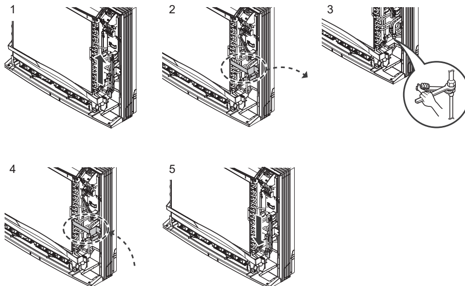
Figure 109: Pipe Connection.
