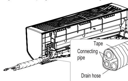
Figure 82: Piping Installed to the Right.
