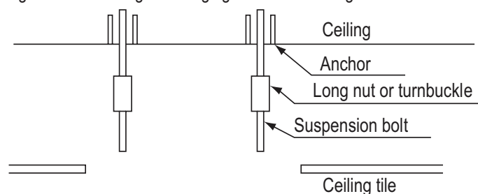
Figure 197: Installing the Hanging Bolt in the Ceiling.
