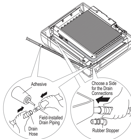
Figure 42: Preparing the Drain Hose.
