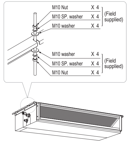
Figure 134:Hanging the Indoor Unit.
