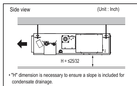
Figure 129: Service / Access Panel Dimensions.
