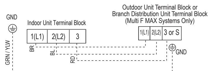
Figure 84: Simplified View of Indoor Unit to Outdoor Unit / Branch Distribution Unit Terminal Connections—LMN079HVT, LSN090HSV5, LSN120HSV5 and LMN159HVT.
