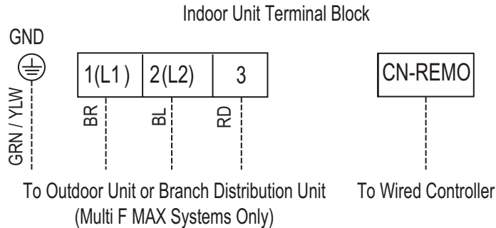
Figure 54: Wired Controller Connection on the Indoor Unit Terminal Block.
