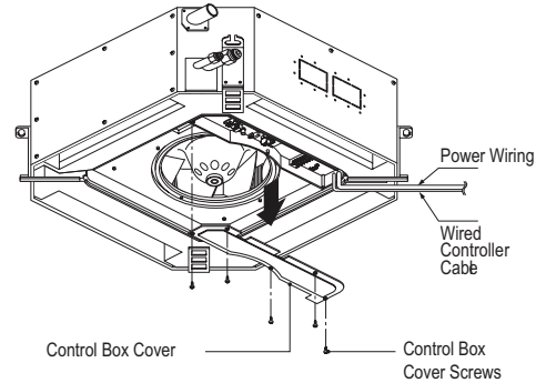
Figure 203: Power Wiring and Communications Cable Connection Access.
