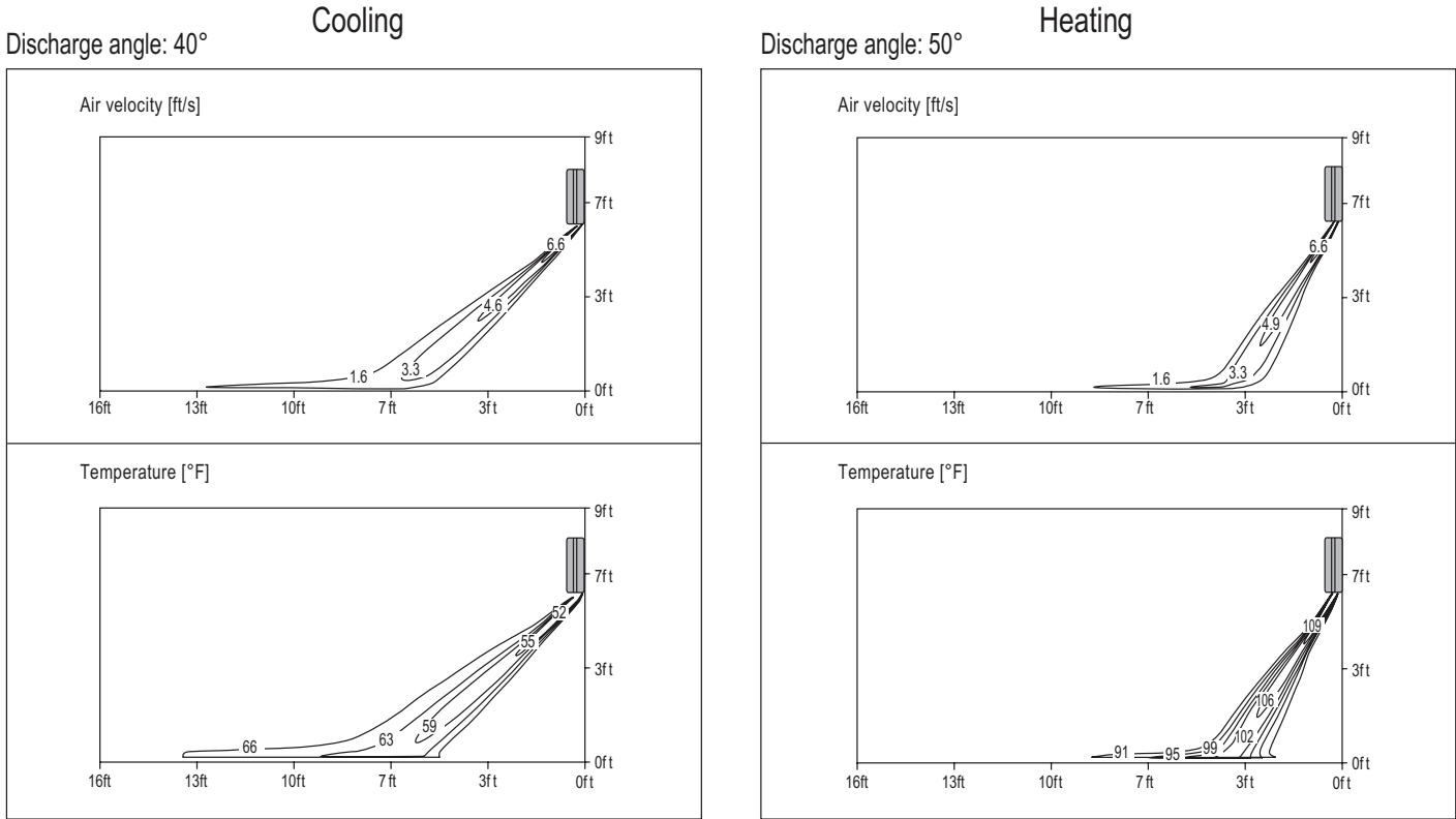
Figure 35: LMAN127HVP Air Velocity and Temperature Distribution Charts.
