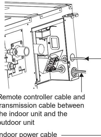
Figure 171: Exterior View of Conduit Installation.
