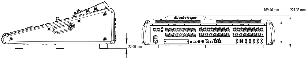
Side view
