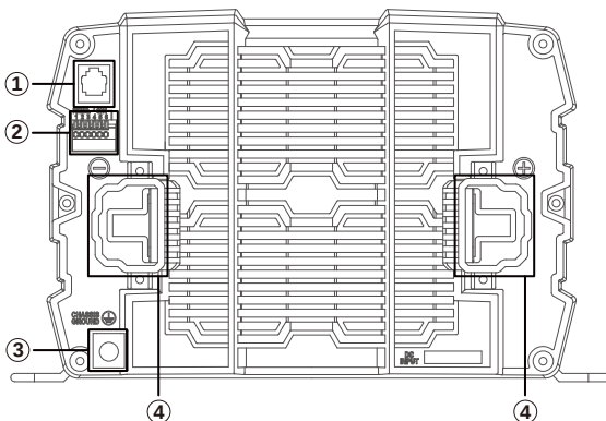
Figure 14. SP-3000/4000
