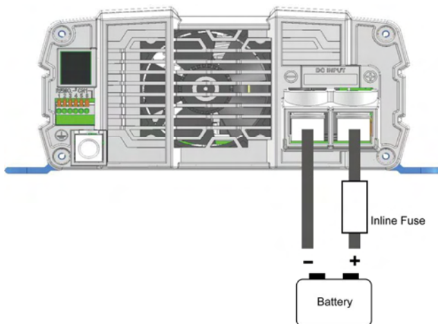
Figure 18. Battery cabling
