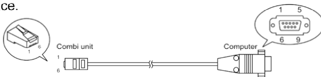
Figure 19. RS-232 cable
