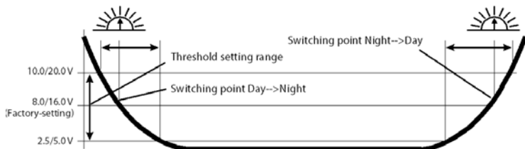
Open circuit voltage curve of solar array
