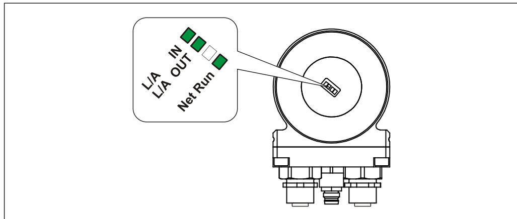
Figure 9: EtherCAT diagnostic LEDs
