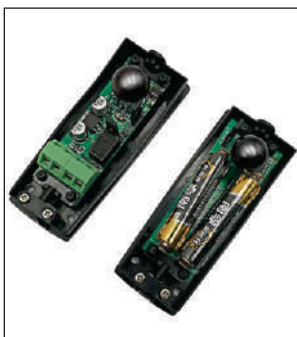
Beam Sensor AAA Battery Operated
