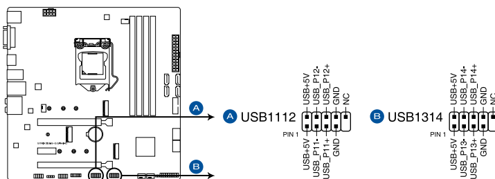
ROG STRIX B365-G GAMING USB 2.0 connector
