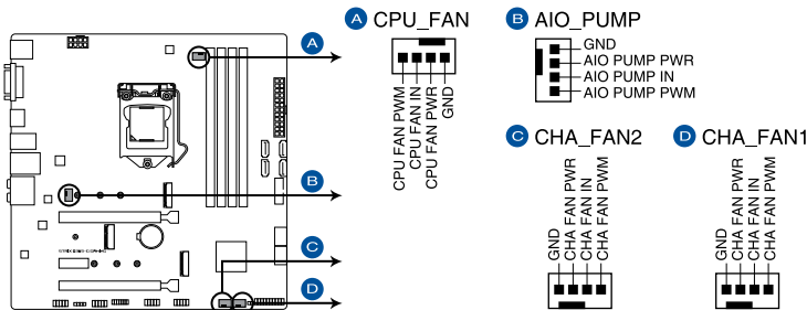
ROG STRIX B365-G GAMING Fan and Pump connectors
