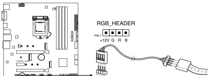
ROG STRIX B365-G GAMING AURA RGB LED connector
