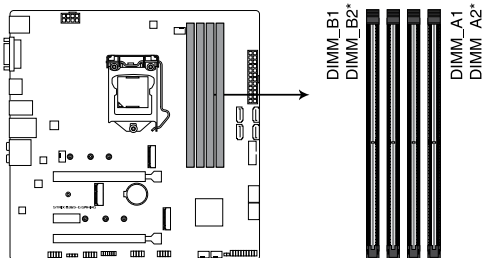
ROG STRIX B365-G GAMING 288-pin DDR4 DIMM socket
