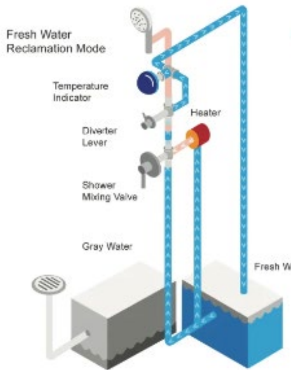
Figure 9-5: ShowerMiser
