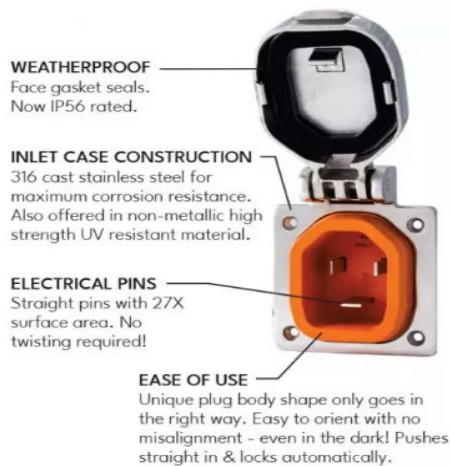
Figure 6-1: SmartPlug
