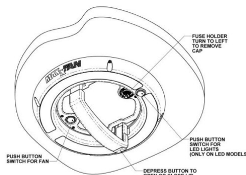
Figure 9-3: Maxxfan Exhaust
