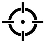
Accept Cursor
