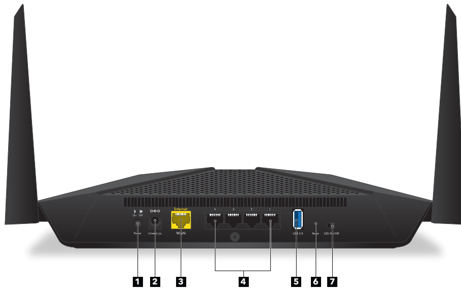
Figure 3. Rear panel
